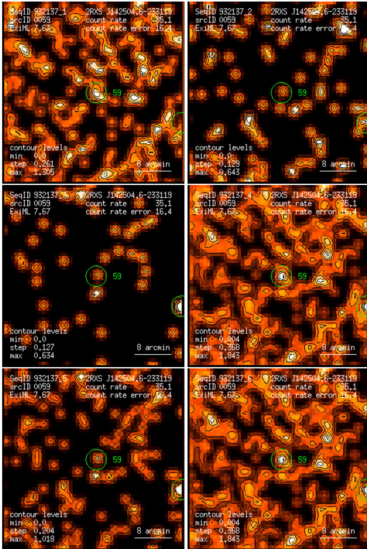
Figure 59: RASS 932137: detection 0059: band rate images, Gaussian filter: (1) PSPC channels 11 – 41, (2) 52 – 90, (3) 91 – 201, (4) 11 – 235, (5) 52 – 201, (6) 11 – 201. Broad band rates in counts/ks. Band rate contour levels in counts/ks/arcmin 2 .
