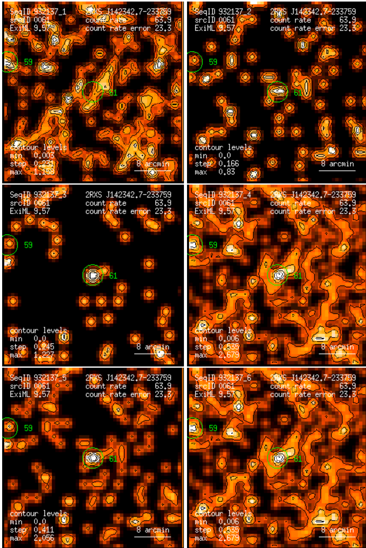
Figure 61: RASS 932137: detection 0061: band rate images, Gaussian filter: (1) PSPC channels 11 – 41, (2) 52 – 90, (3) 91 – 201, (4) 11 – 235, (5) 52 – 201, (6) 11 – 201. Broad band rates in counts/ks. Band rate contour levels in counts/ks/arcmin 2 .
