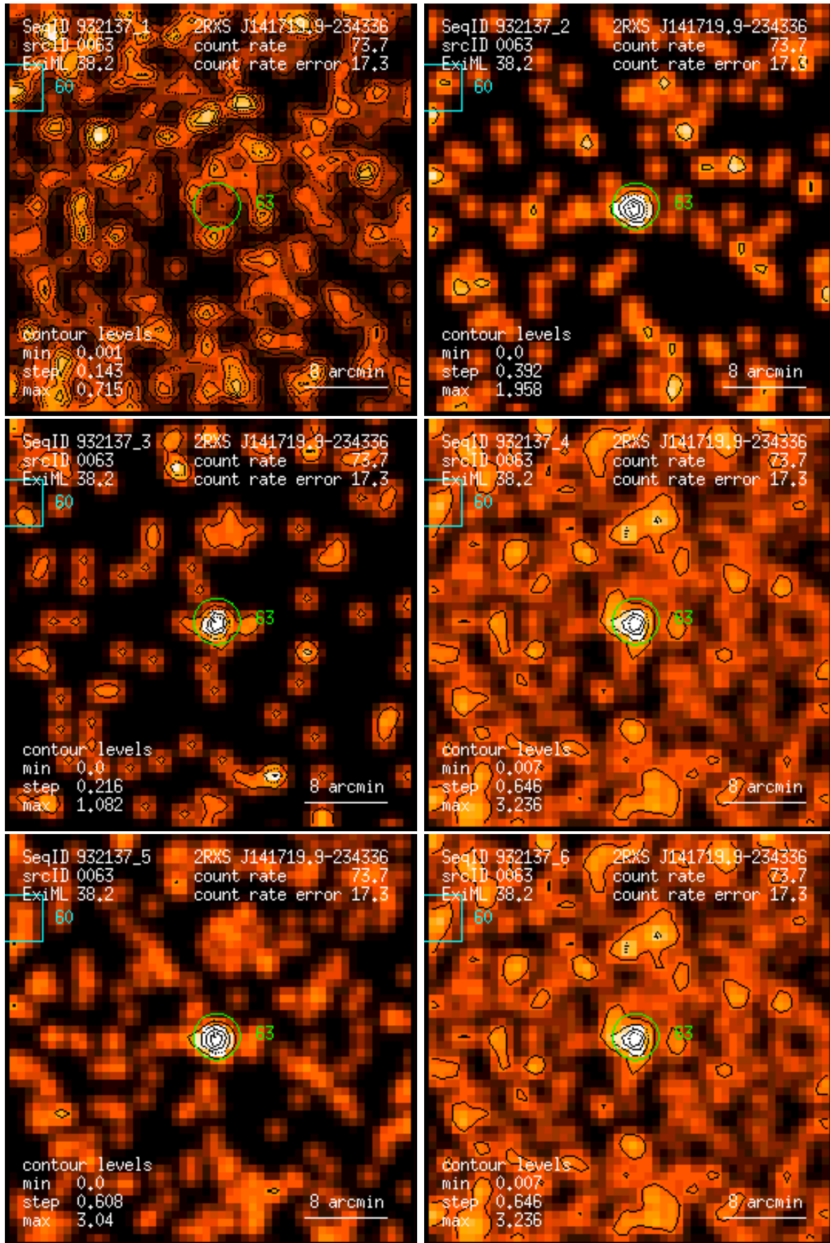
Figure 63: RASS 932137: detection 0063: band rate images, Gaussian filter: (1) PSPC channels 11 – 41, (2) 52 – 90, (3) 91 – 201, (4) 11 – 235, (5) 52 – 201, (6) 11 – 201. Broad band rates in counts/ks. Band rate contour levels in counts/ks/arcmin 2 .
