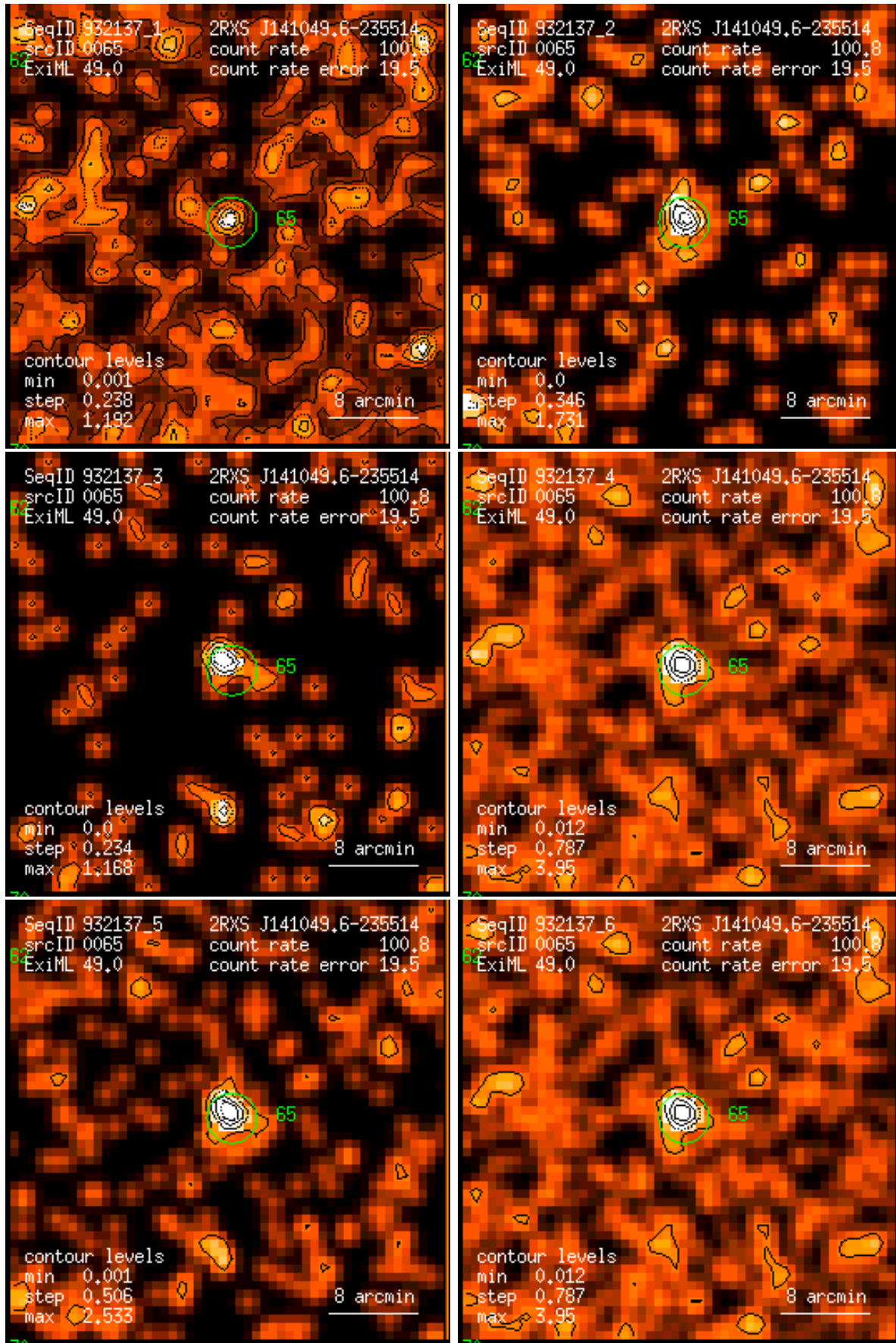
Figure 65: RASS 932137: detection 0065: band rate images, Gaussian filter: (1) PSPC channels 11 – 41, (2) 52 – 90, (3) 91 – 201, (4) 11 – 235, (5) 52 – 201, (6) 11 – 201. Broad band rates in counts/ks. Band rate contour levels in counts/ks/arcmin 2 .
