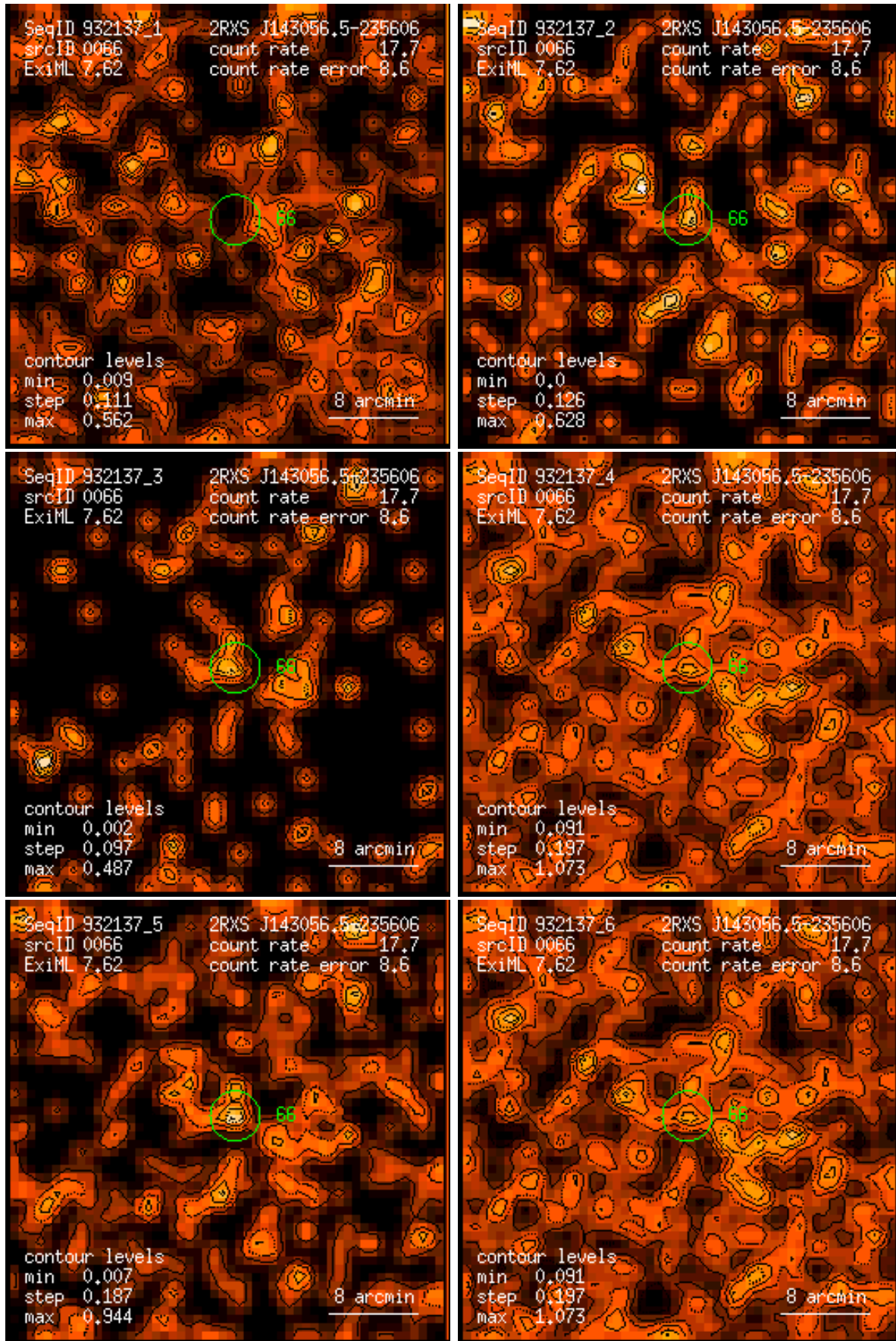
Figure 66: RASS 932137: detection 0066: band rate images, Gaussian filter: (1) PSPC channels 11 – 41, (2) 52 – 90, (3) 91 – 201, (4) 11 – 235, (5) 52 – 201, (6) 11 – 201. Broad band rates in counts/ks. Band rate contour levels in counts/ks/arcmin 2 .
