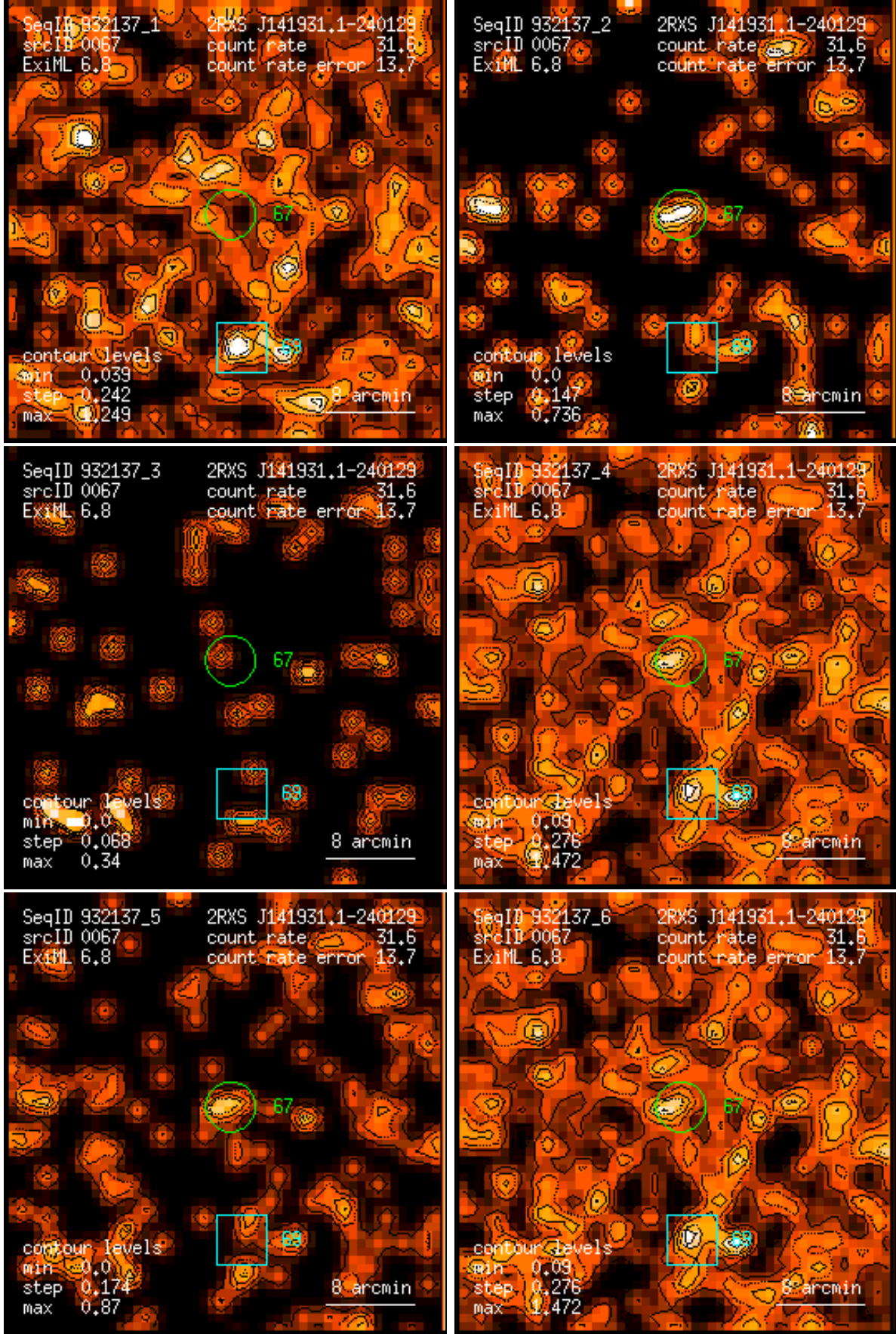
Figure 67: RASS 932137: detection 0067: band rate images, Gaussian filter: (1) PSPC channels 11 – 41, (2) 52 – 90, (3) 91 – 201, (4) 11 – 235, (5) 52 – 201, (6) 11 – 201. Broad band rates in counts/ks. Band rate contour levels in counts/ks/arcmin 2 .
