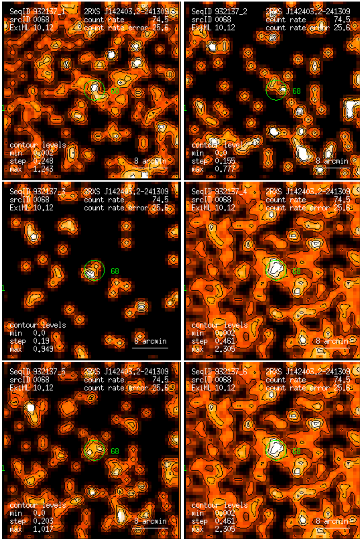
Figure 68: RASS 932137: detection 0068: band rate images, Gaussian filter: (1) PSPC channels 11 – 41, (2) 52 – 90, (3) 91 – 201, (4) 11 – 235, (5) 52 – 201, (6) 11 – 201. Broad band rates in counts/ks. Band rate contour levels in counts/ks/arcmin 2 .
