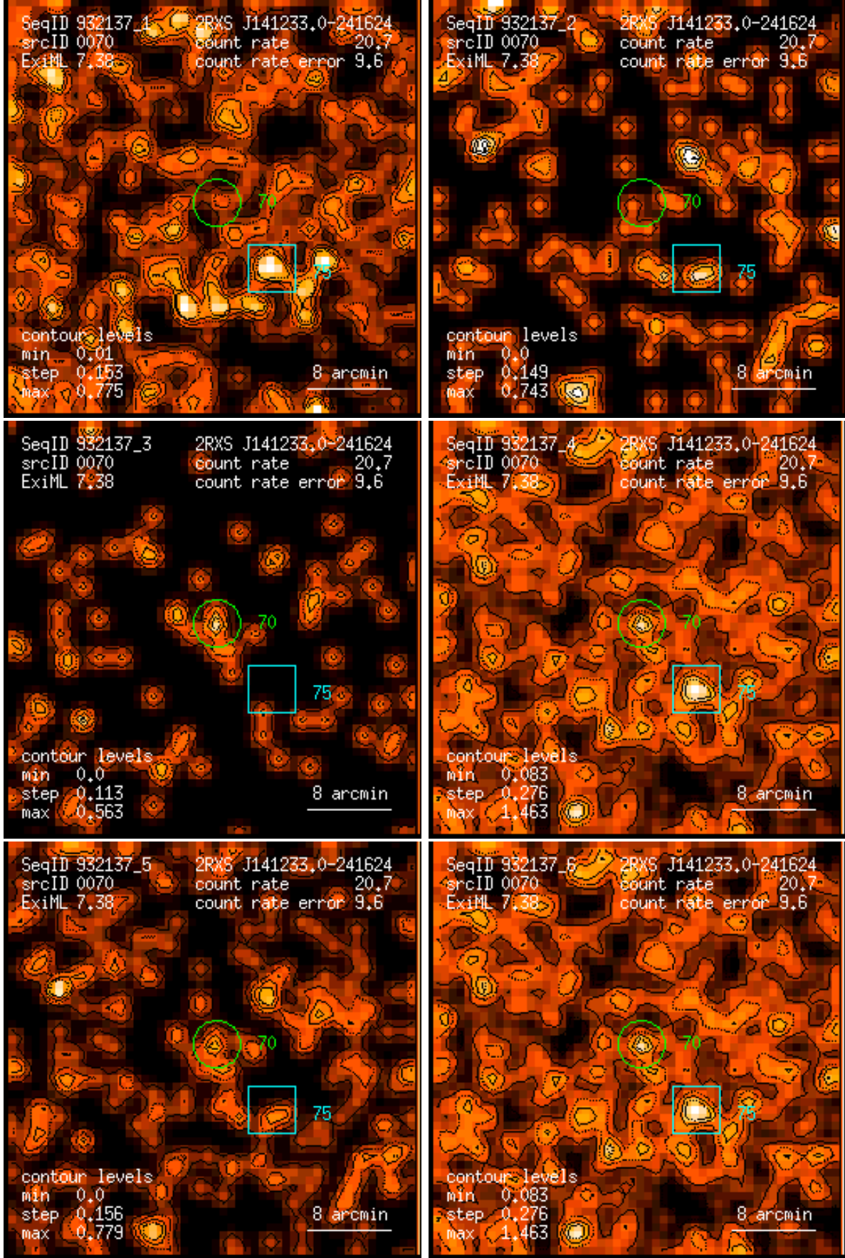
Figure 70: RASS 932137: detection 0070: band rate images, Gaussian filter: (1) PSPC channels 11 – 41, (2) 52 – 90, (3) 91 – 201, (4) 11 – 235, (5) 52 – 201, (6) 11 – 201. Broad band rates in counts/ks. Band rate contour levels in counts/ks/arcmin 2 .
