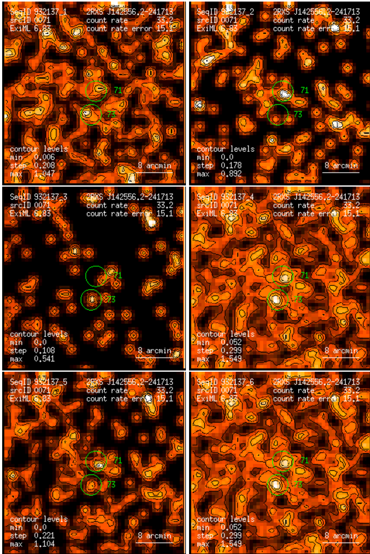
Figure 71: RASS 932137: detection 0071: band rate images, Gaussian filter: (1) PSPC channels 11 – 41, (2) 52 – 90, (3) 91 – 201, (4) 11 – 235, (5) 52 – 201, (6) 11 – 201. Broad band rates in counts/ks. Band rate contour levels in counts/ks/arcmin 2 .
