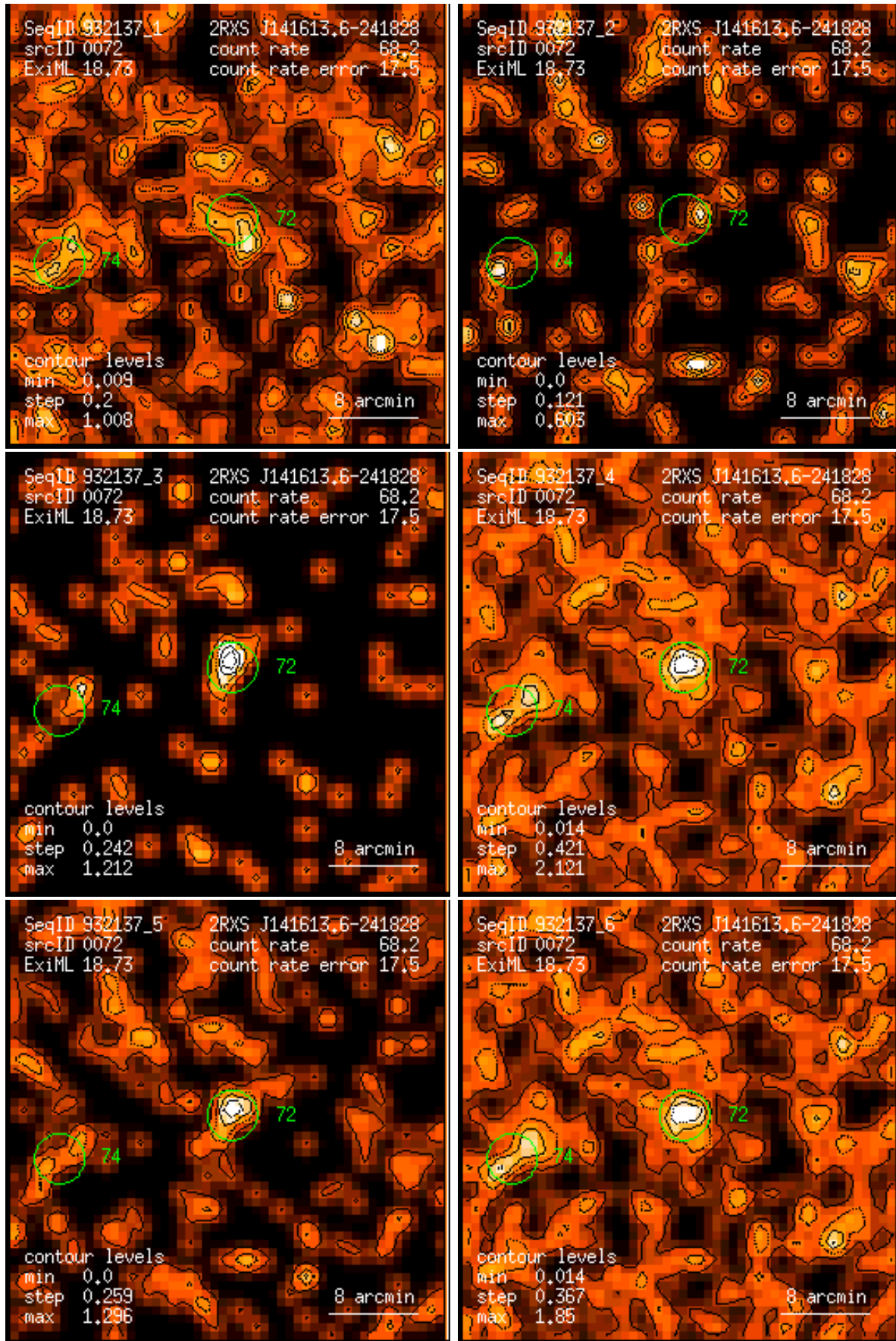
Figure 72: RASS 932137: detection 0072: band rate images, Gaussian filter: (1) PSPC channels 11 – 41, (2) 52 – 90, (3) 91 – 201, (4) 11 – 235, (5) 52 – 201, (6) 11 – 201. Broad band rates in counts/ks. Band rate contour levels in counts/ks/arcmin 2 .
