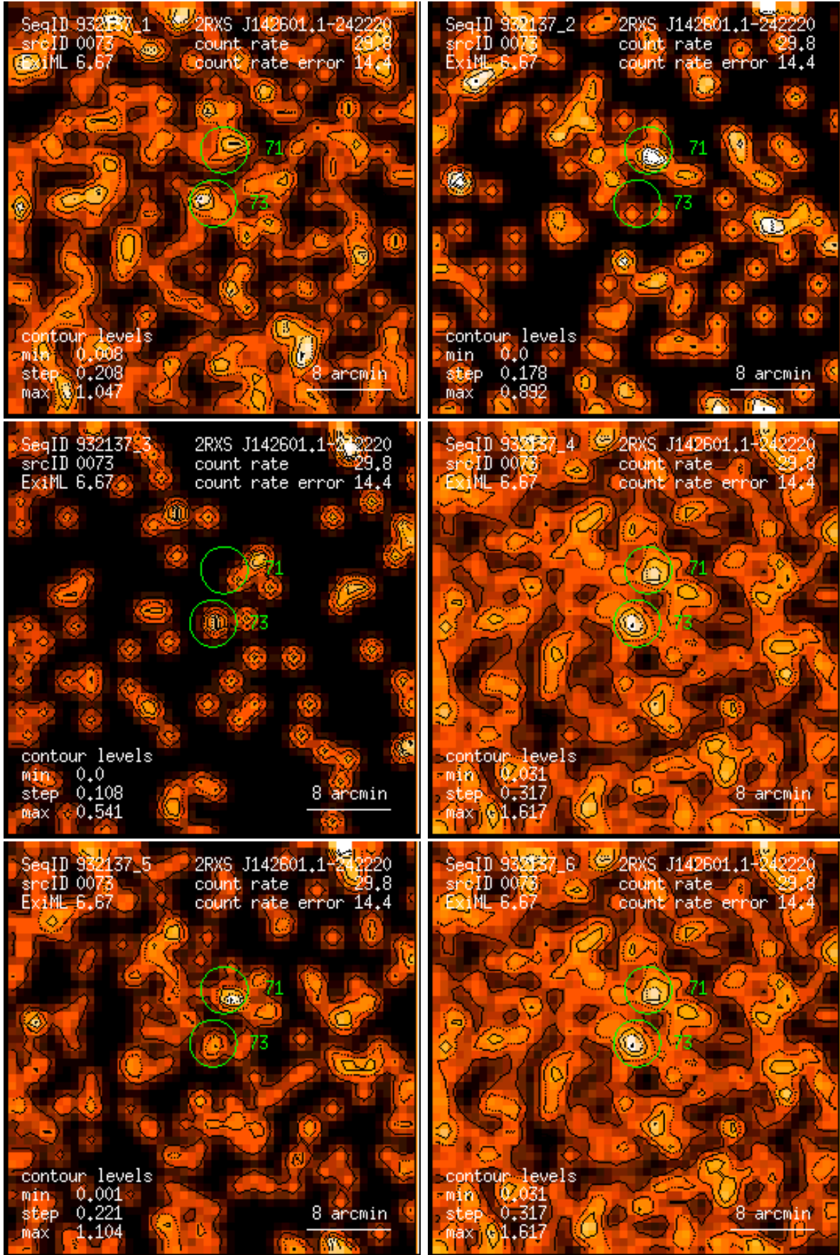
Figure 73: RASS 932137: detection 0073: band rate images, Gaussian filter: (1) PSC channels 11 – 41, (2) 52 – 90, (3) 91 – 201, (4) 11 – 235, (5) 52 – 201, (6) 11 – 201. Broad band rates in counts/ks. Band rate contour levels in counts/ks/arcmin 2 .
