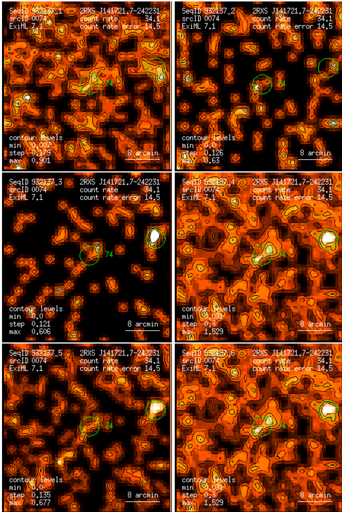
Figure 74: RASS 932137: detection 0074: band rate images, Gaussian filter: (1) PSPC channels 11 – 41, (2) 52 – 90, (3) 91 – 201, (4) 11 – 235, (5) 52 – 201, (6) 11 – 201. Broad band rates in counts/ks. Band rate contour levels in counts/ks/arcmin 2 .
