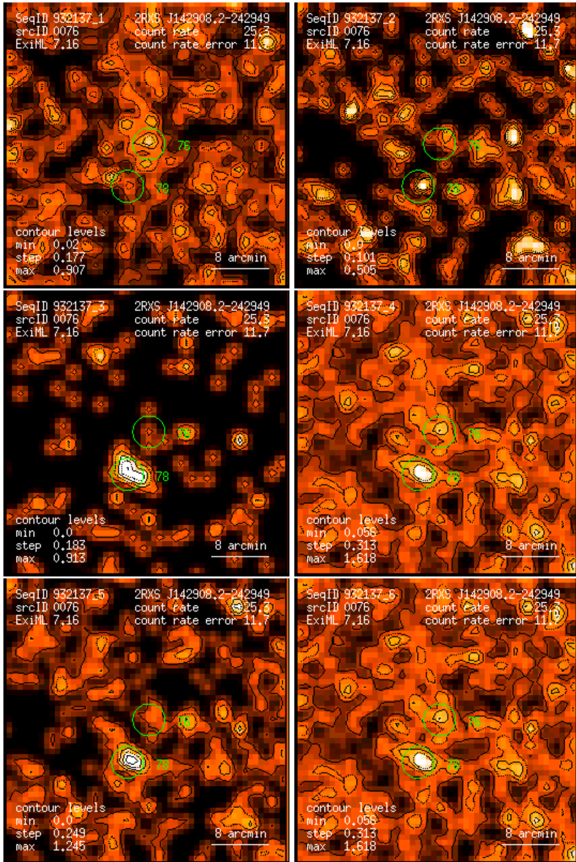
Figure 76: RASS 932137: detection 0076: band rate images, Gaussian filter: (1) PSPC channels 11 – 41, (2) 52 – 90, (3) 91 – 201, (4) 11 – 235, (5) 52 – 201, (6) 11 – 201. Broad band rates in counts/ks. Band rate contour levels in counts/ks/arcmin 2 .
