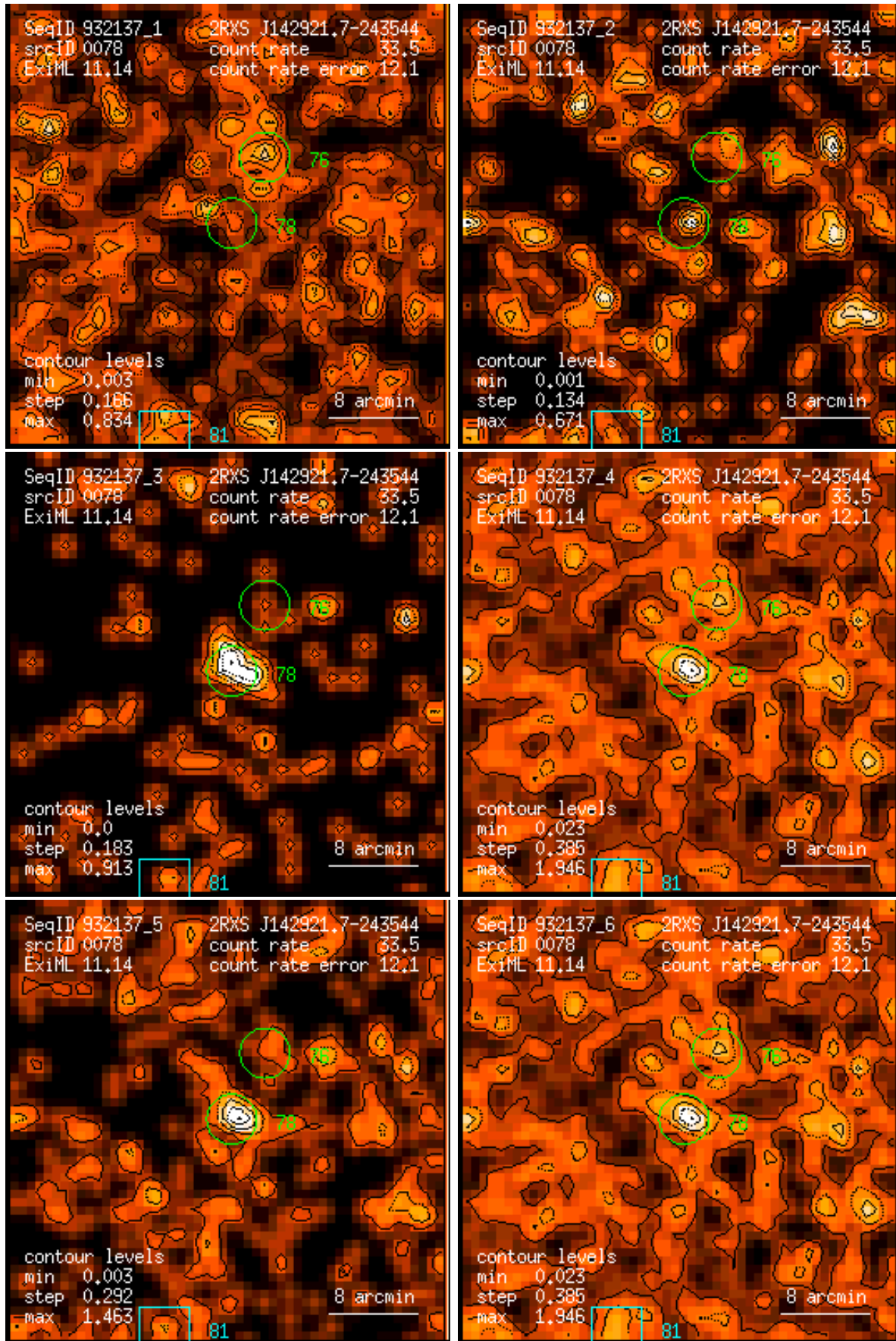
Figure 78: RASS 932137: detection 0078: band rate images, Gaussian filter: (1) PSPC channels 11 – 41, (2) 52 – 90, (3) 91 – 201, (4) 11 – 235, (5) 52 – 201, (6) 11 – 201. Broad band rates in counts/ks. Band rate contour levels in counts/ks/arcmin 2 .
