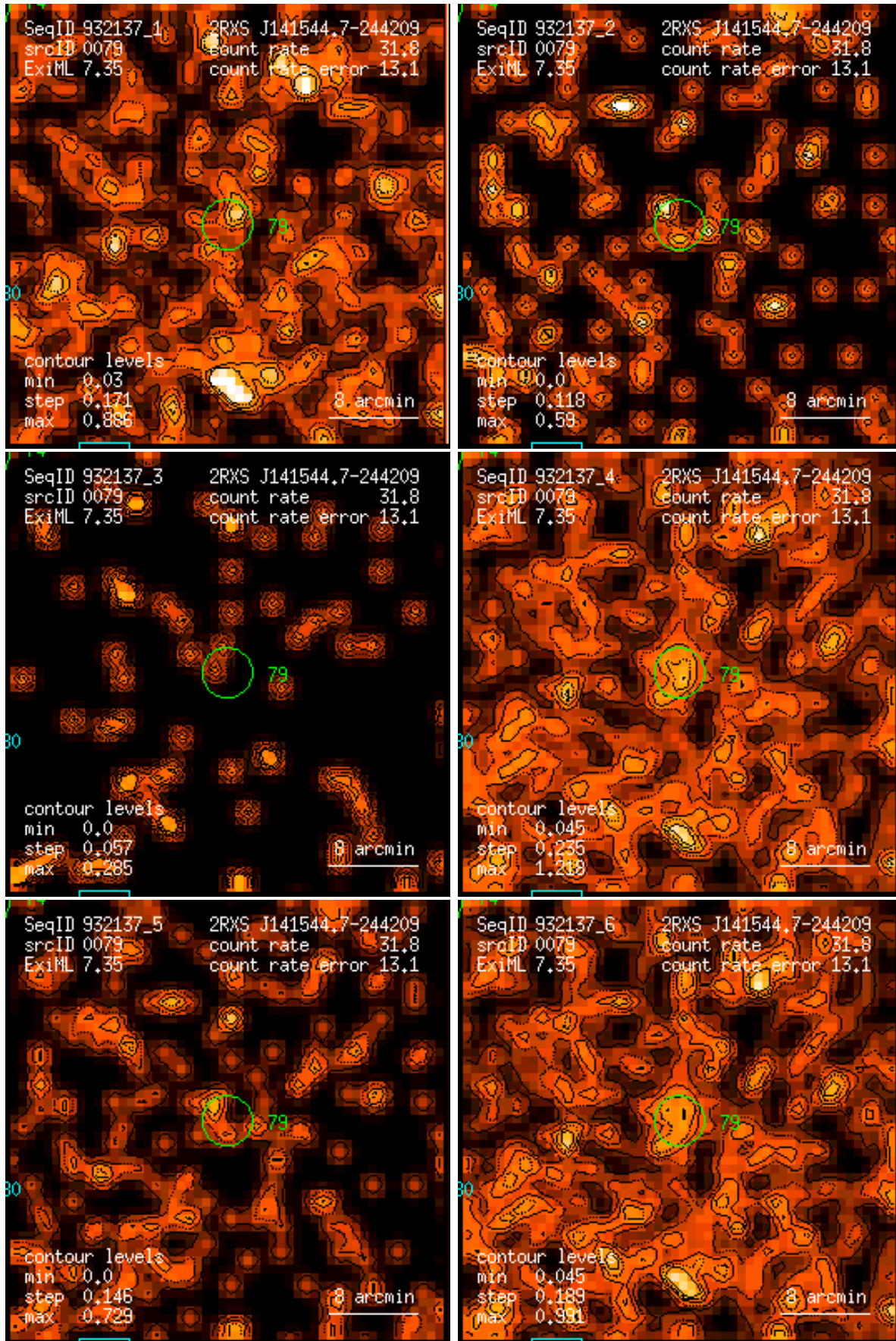
Figure 79: RASS 932137: detection 0079: band rate images, Gaussian filter: (1) PSPC channels 11 – 41, (2) 52 – 90, (3) 91 – 201, (4) 11 – 235, (5) 52 – 201, (6) 11 – 201. Broad band rates in counts/ks. Band rate contour levels in counts/ks/arcmin 2 .
