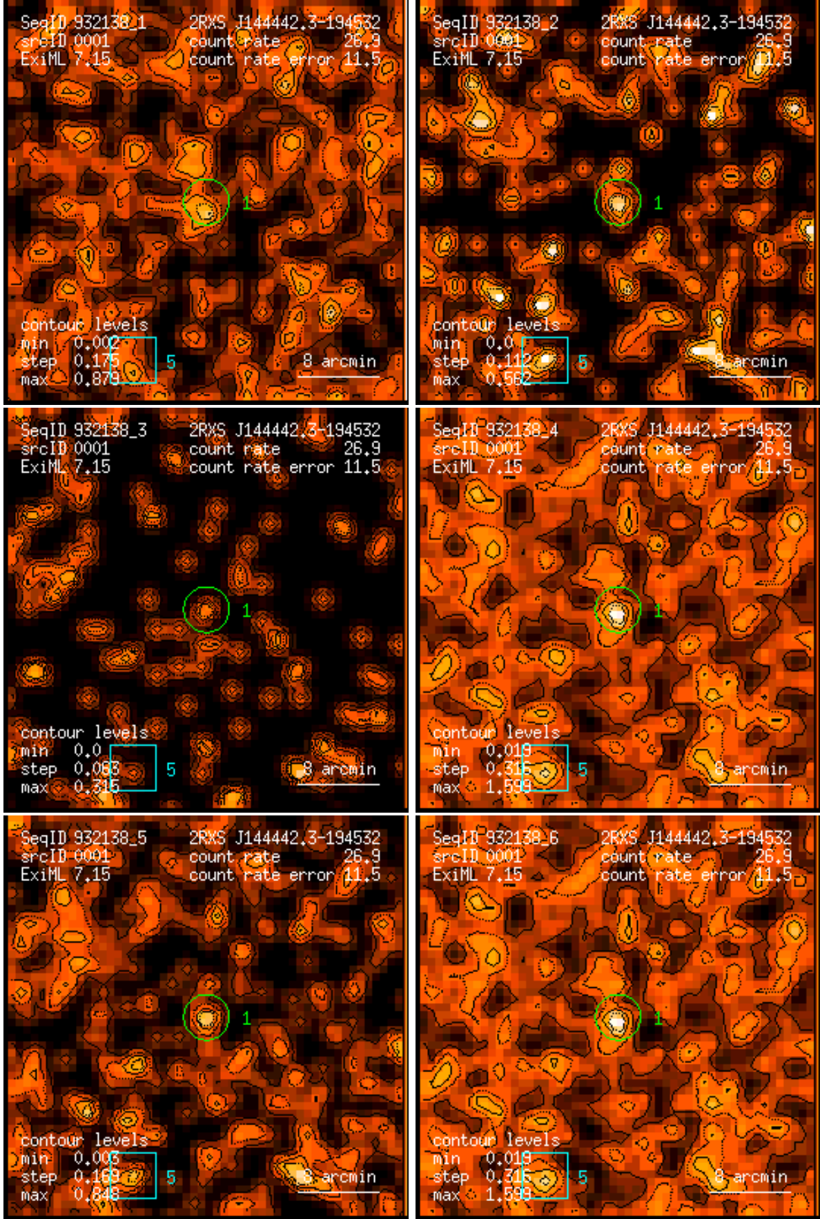
Figure 1: RASS 932138: detection 0001: band rate images, Gaussian filter: (1) PSPC channels 11 – 41, (2) 52 – 90, (3) 91 – 201, (4) 11 – 235, (5) 52 – 201, (6) 11 – 201. Broad band rates in counts/ks. Band rate contour levels in counts/ks/arcmin 2 .
