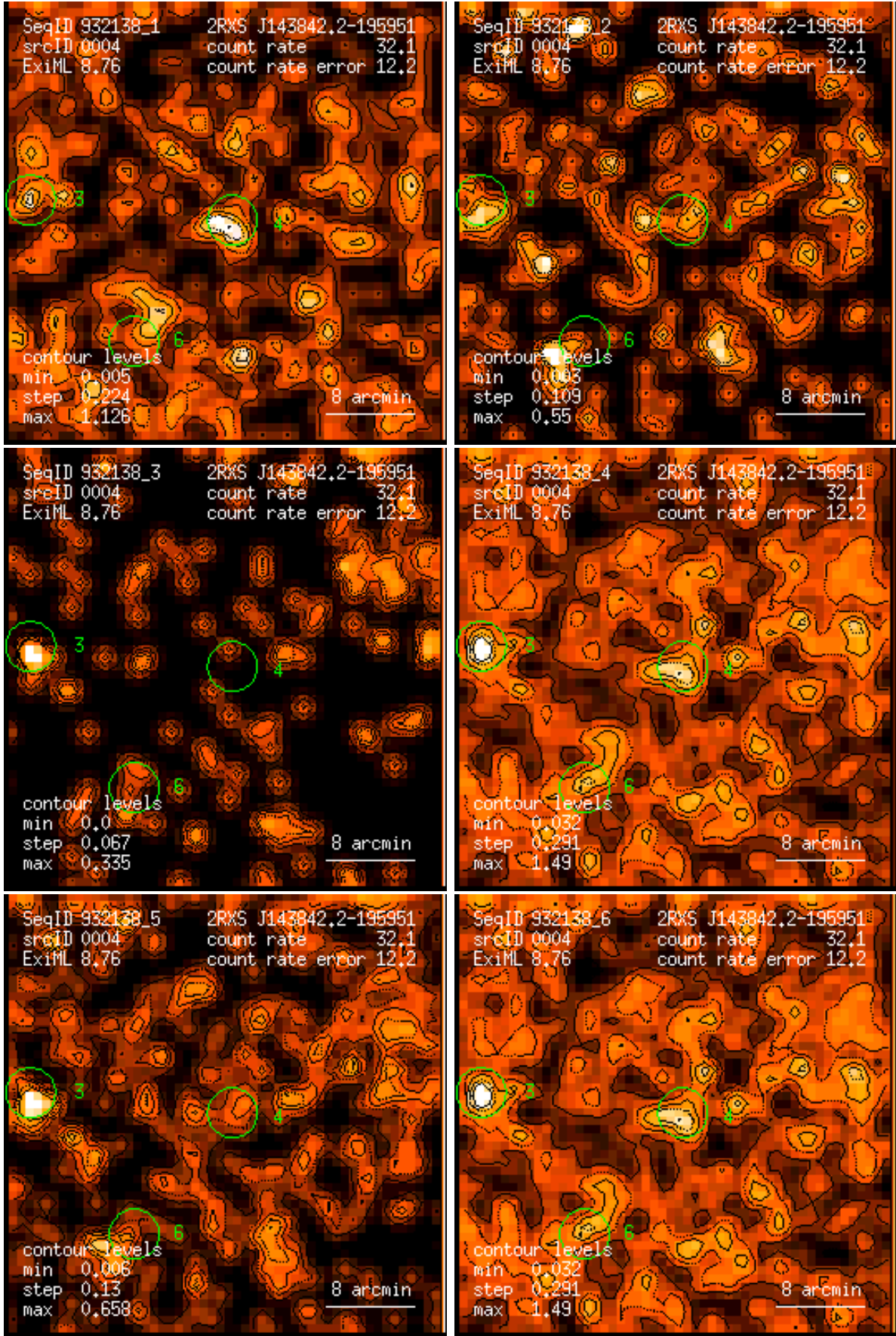
Figure 4: RASS 932138: detection 0004: band rate images, Gaussian filter: (1) PSPC channels 11 – 41, (2) 52 – 90, (3) 91 – 201, (4) 11 – 235, (5) 52 – 201, (6) 11 – 201. Broad band rates in counts/ks. Band rate contour levels in counts/ks/arcmin 2 .
