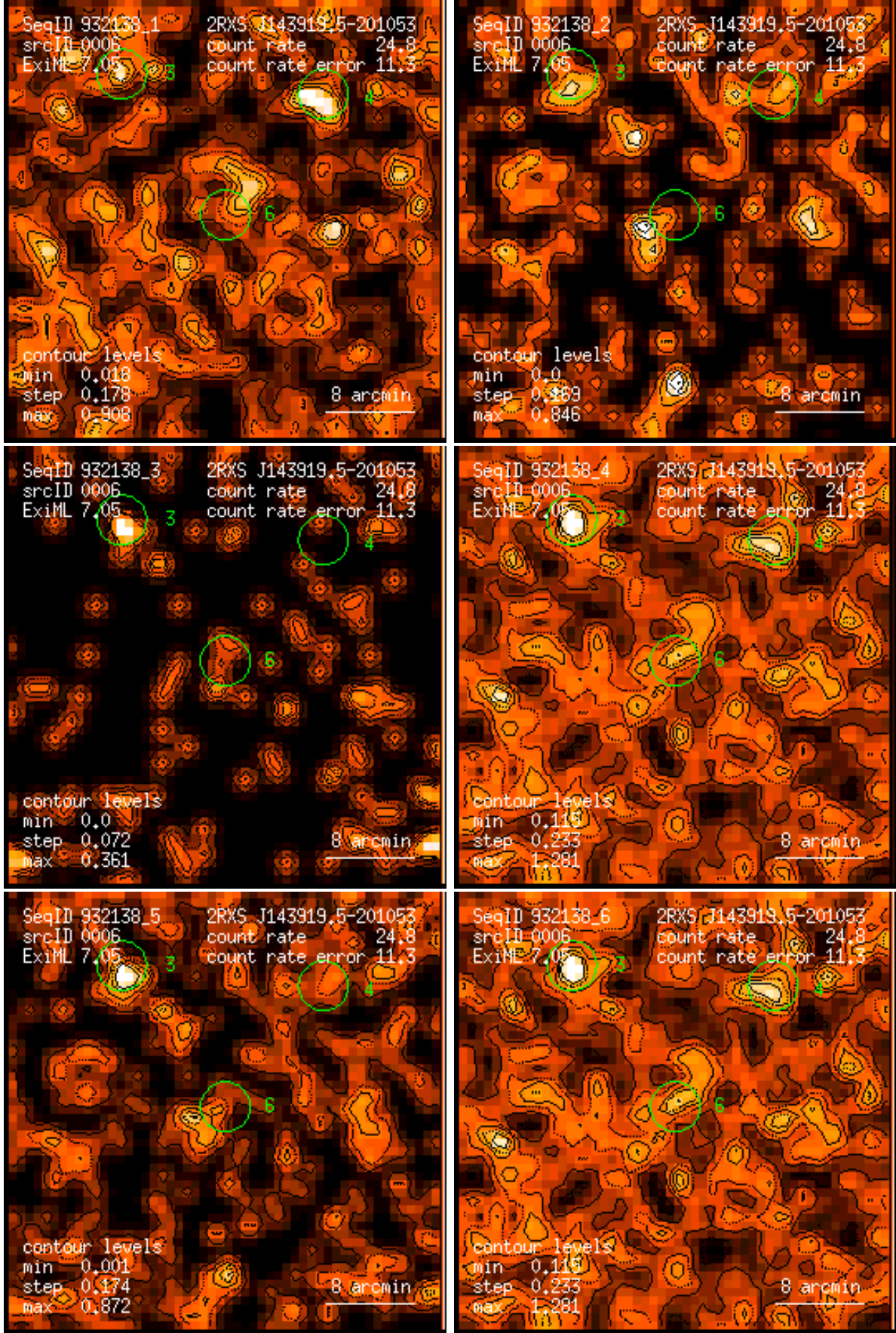
Figure 6: RASS 932138: detection 0006: band rate images, Gaussian filter: (1) PSPC channels 11 – 41, (2) 52 – 90, (3) 91 – 201, (4) 11 – 235, (5) 52 – 201, (6) 11 – 201. Broad band rates in counts/ks. Band rate contour levels in counts/ks/arcmin 2 .
