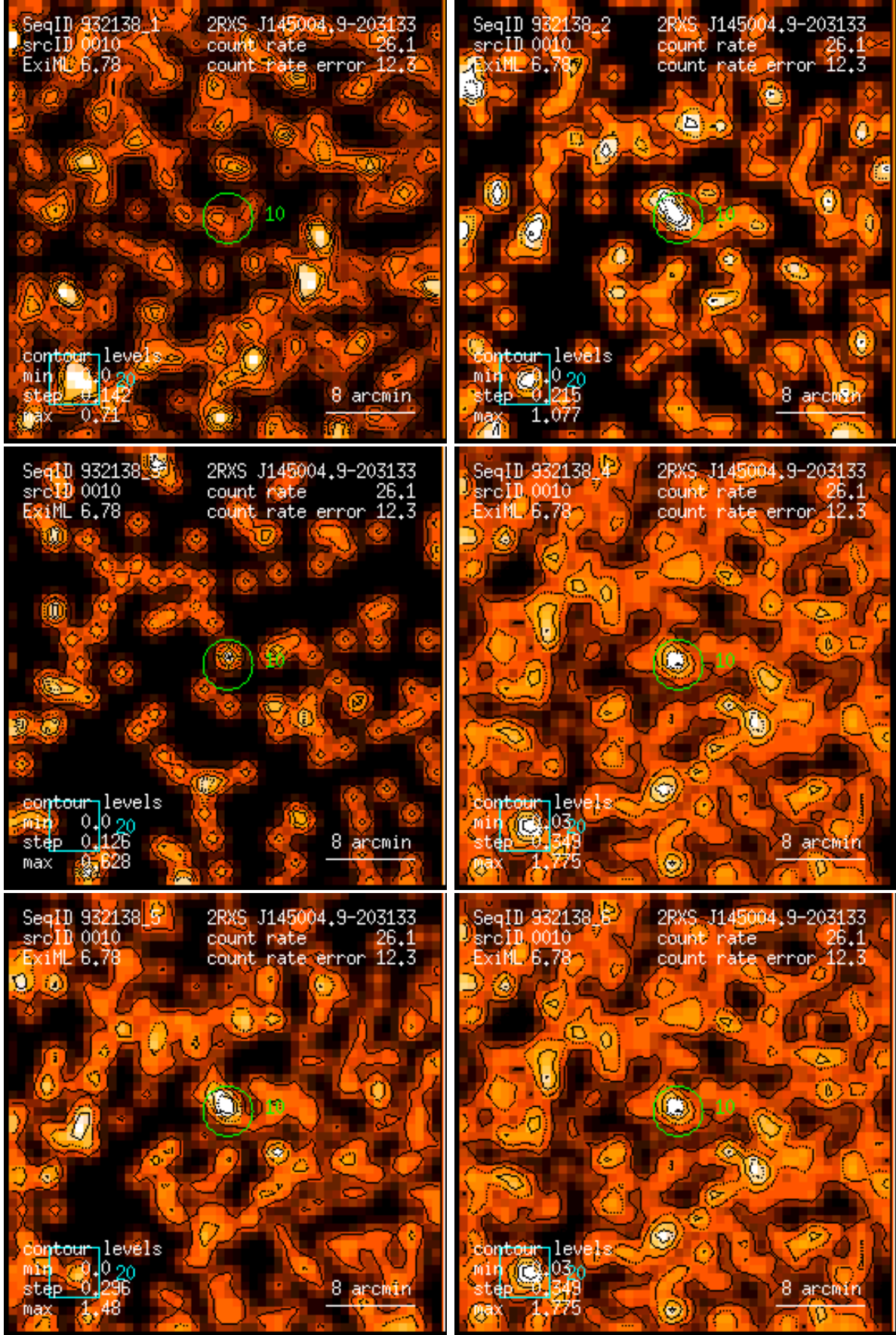
Figure 10: RASS 932138: detection 0010: band rate images, Gaussian filter: (1) PSPC channels 11 – 41, (2) 52 – 90, (3) 91 – 201, (4) 11 – 235, (5) 52 – 201, (6) 11 – 201. Broad band rates in counts/ks. Band rate contour levels in counts/ks/arcmin 2 .
