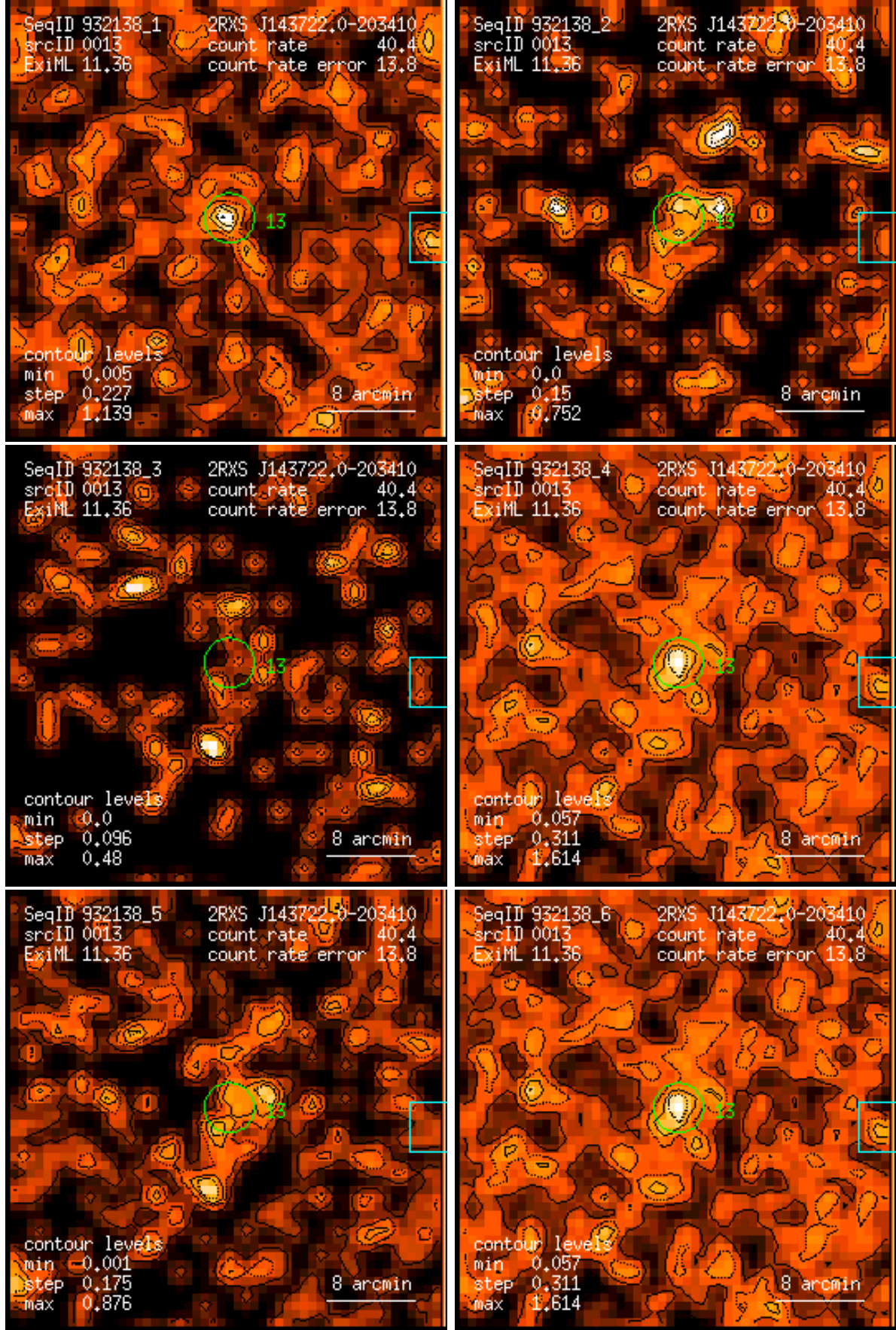
Figure 13: RASS 932138: detection 0013: band rate images, Gaussian filter: (1) PSPC channels 11 – 41, (2) 52 – 90, (3) 91 – 201, (4) 11 – 235, (5) 52 – 201, (6) 11 – 201. Broad band rates in counts/ks. Band rate contour levels in counts/ks/arcmin 2 .
