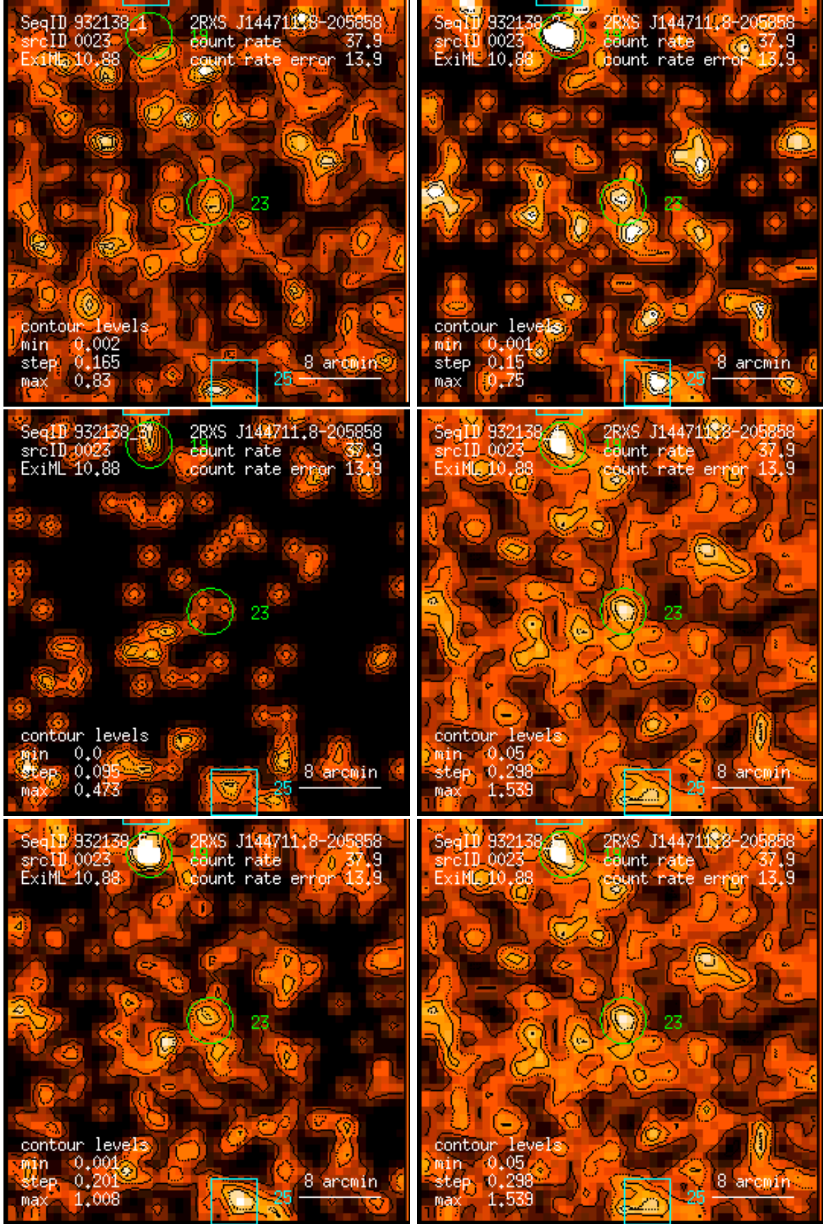
Figure 23: RASS 932138: detection 0023: band rate images, Gaussian filter: (1) PSPC channels 11 – 41, (2) 52 – 90, (3) 91 – 201, (4) 11 – 235, (5) 52 – 201, (6) 11 – 201. Broad band rates in counts/ks. Band rate contour levels in counts/ks/arcmin 2 .
