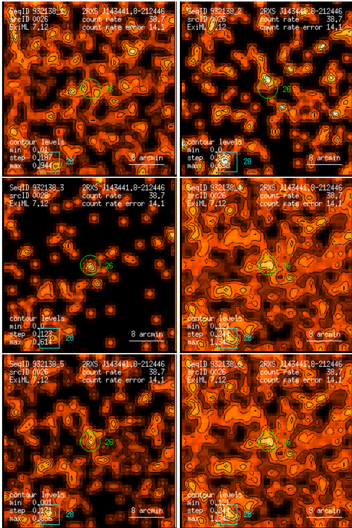
Figure 26: RASS 932138: detection 0026: band rate images, Gaussian filter: (1) PSPC channels 11 – 41, (2) 52 – 90, (3) 91 – 201, (4) 11 – 235, (5) 52 – 201, (6) 11 – 201. Broad band rates in counts/ks. Band rate contour levels in counts/ks/arcmin 2 .
