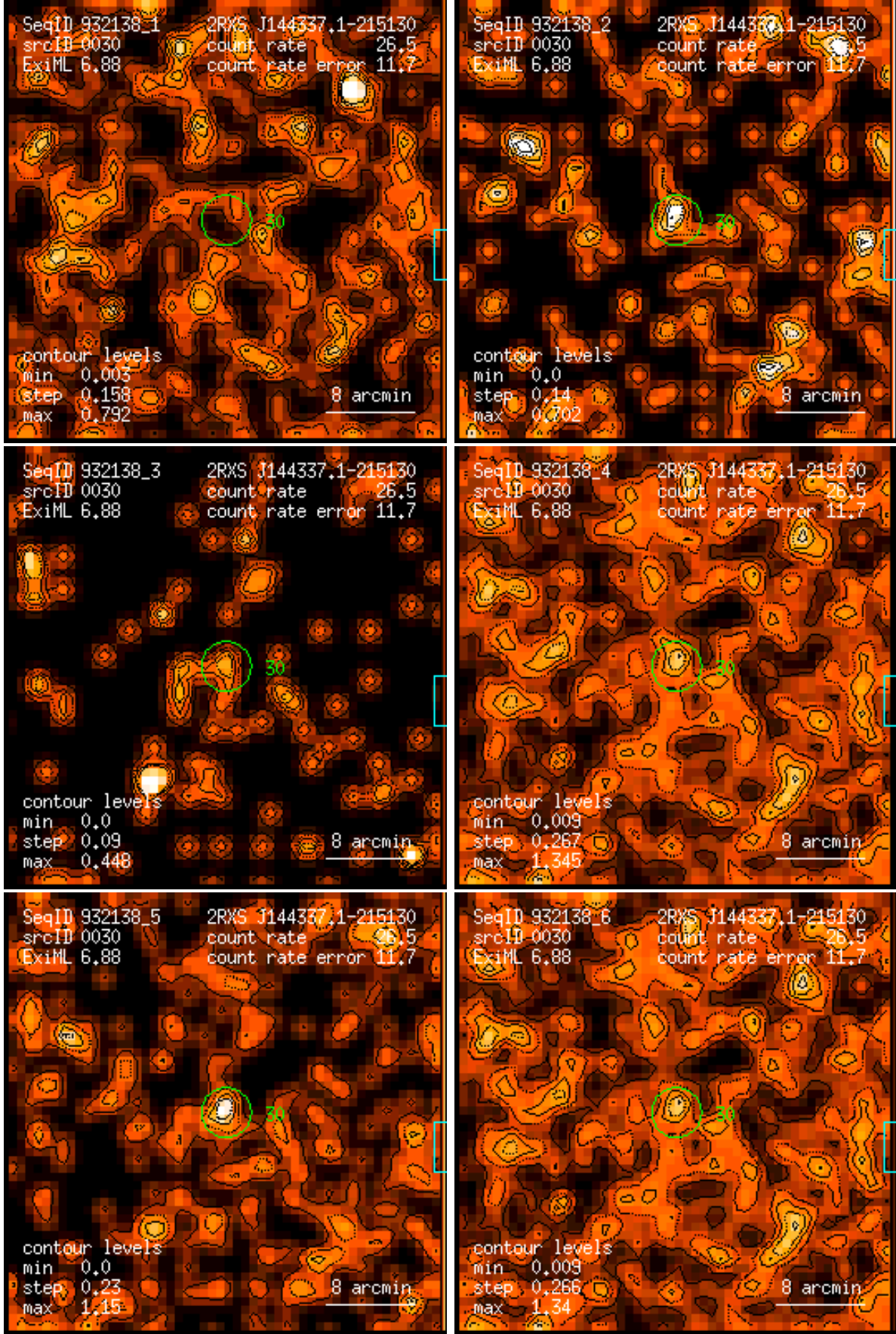
Figure 30: RASS 932138: detection 0030: band rate images, Gaussian filter: (1) PSPC channels 11 – 41, (2) 52 – 90, (3) 91 – 201, (4) 11 – 235, (5) 52 – 201, (6) 11 – 201. Broad band rates in counts/ks. Band rate contour levels in counts/ks/arcmin 2 .
