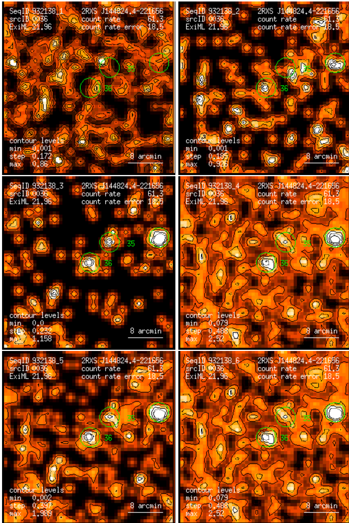
Figure 36: RASS 932138: detection 0036: band rate images, Gaussian filter: (1) PSPC channels 11 – 41, (2) 52 – 90, (3) 91 – 201, (4) 11 – 235, (5) 52 – 201, (6) 11 – 201. Broad band rates in counts/ks. Band rate contour levels in counts/ks/arcmin 2 .
