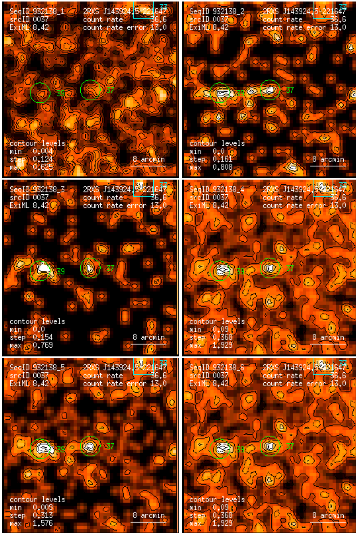
Figure 37: RASS 932138: detection 0037: band rate images, Gaussian filter: (1) PSPC channels 11 – 41, (2) 52 – 90, (3) 91 – 201, (4) 11 – 235, (5) 52 – 201, (6) 11 – 201. Broad band rates in counts/ks. Band rate contour levels in counts/ks/arcmin 2 .
