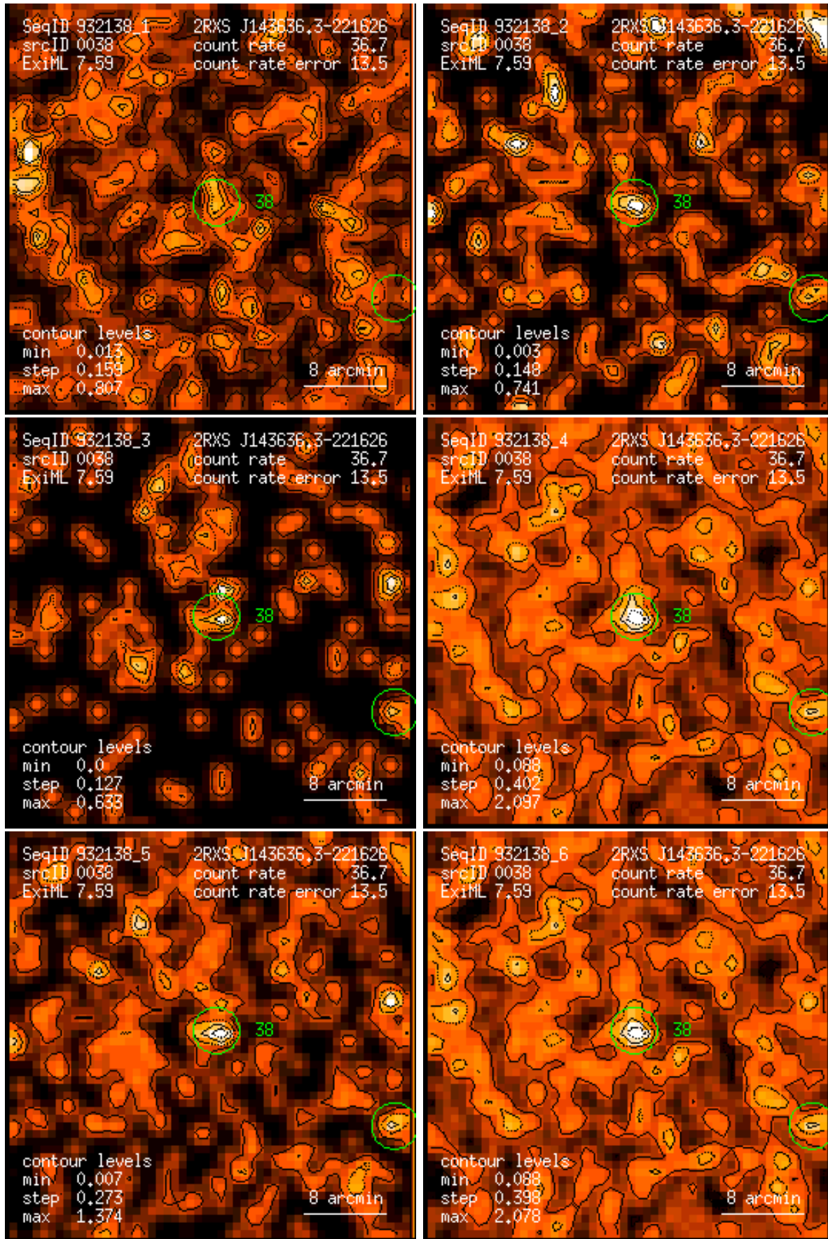
Figure 38: RASS 932138: detection 0038: band rate images, Gaussian filter: (1) PSPC channels 11 – 41, (2) 52 – 90, (3) 91 – 201, (4) 11 – 235, (5) 52 – 201, (6) 11 – 201. Broad band rates in counts/ks. Band rate contour levels in counts/ks/arcmin 2 .
