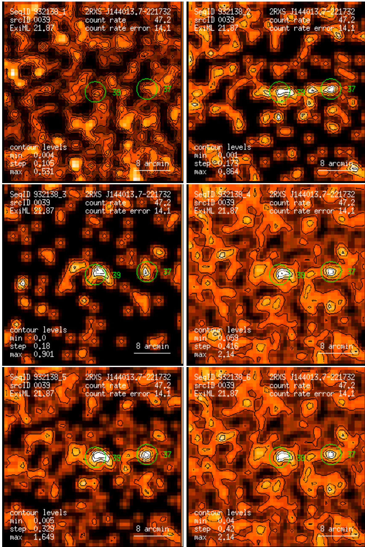
Figure 39: RASS 932138: detection 0039: band rate images, Gaussian filter: (1) PSPC channels 11 – 41, (2) 52 – 90, (3) 91 – 201, (4) 11 – 235, (5) 52 – 201, (6) 11 – 201. Broad band rates in counts/ks. Band rate contour levels in counts/ks/arcmin 2 .
