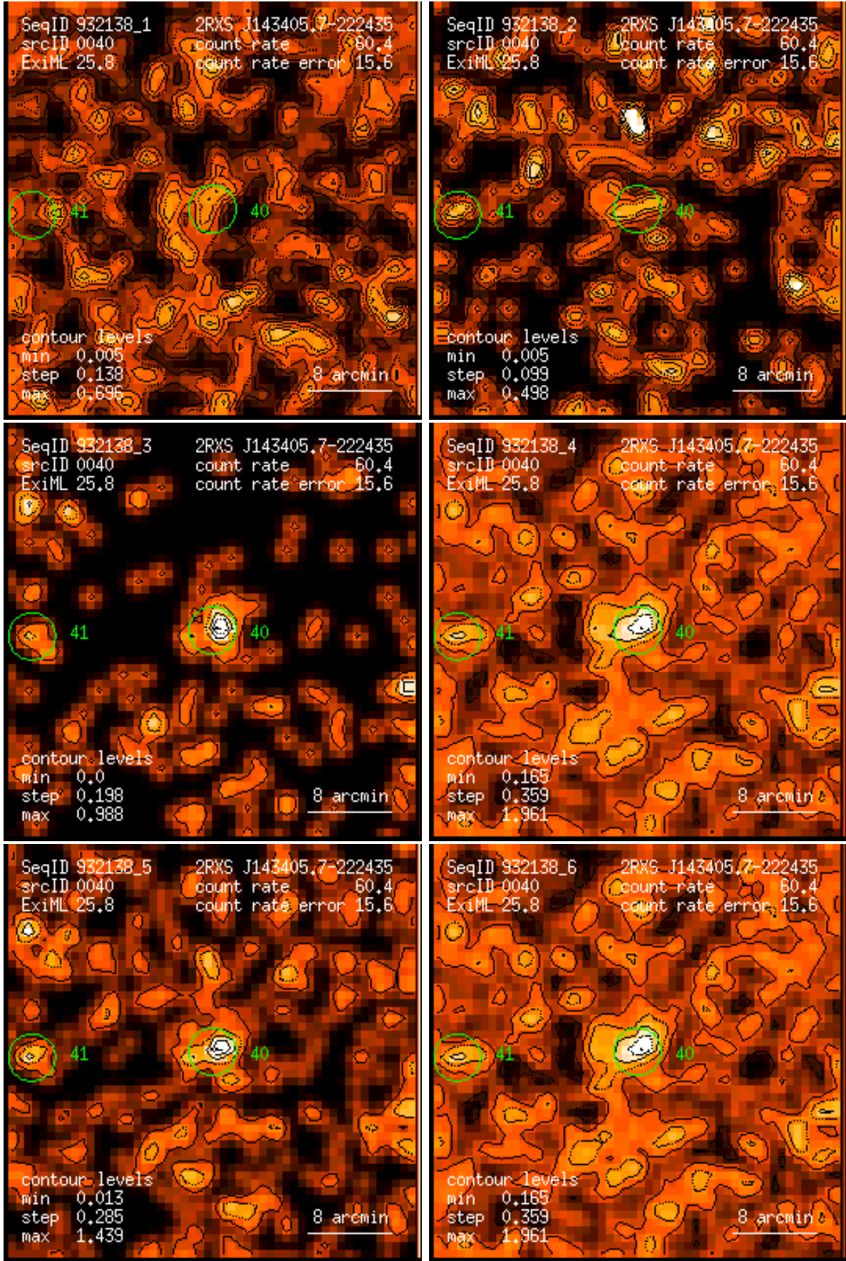
Figure 40: RASS 932138: detection 0040: band rate images, Gaussian filter: (1) PSPC channels 11 – 41, (2) 52 – 90, (3) 91 – 201, (4) 11 – 235, (5) 52 – 201, (6) 11 – 201. Broad band rates in counts/ks. Band rate contour levels in counts/ks/arcmin 2 .
