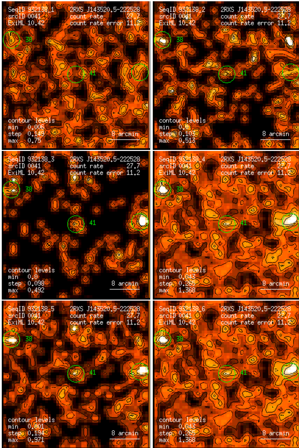
Figure 41: RASS 932138: detection 0041: band rate images, Gaussian filter: (1) PSPC channels 11 – 41, (2) 52 – 90, (3) 91 – 201, (4) 11 – 235, (5) 52 – 201, (6) 11 – 201. Broad band rates in counts/ks. Band rate contour levels in counts/ks/arcmin 2 .
