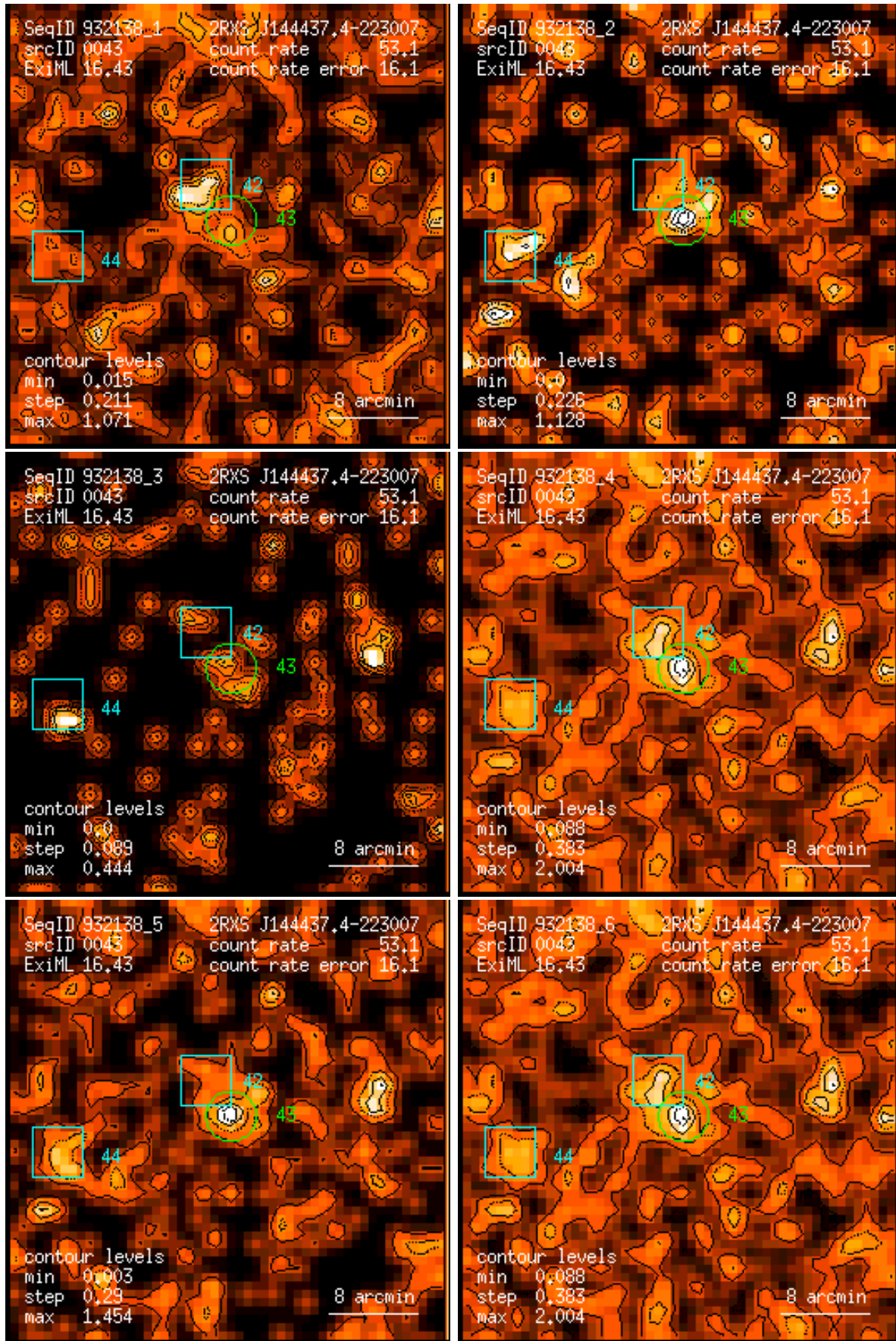
Figure 43: RASS 932138: detection 0043: band rate images, Gaussian filter: (1) PSPC channels 11 – 41, (2) 52 – 90, (3) 91 – 201, (4) 11 – 235, (5) 52 – 201, (6) 11 – 201. Broad band rates in counts/ks. Band rate contour levels in counts/ks/arcmin 2 .
