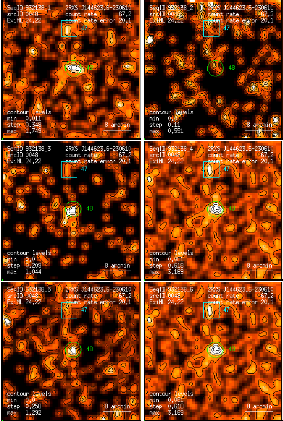
Figure 48: RASS 932138: detection 0048: band rate images, Gaussian filter: (1) PSPC channels 11 – 41, (2) 52 – 90, (3) 91 – 201, (4) 11 – 235, (5) 52 – 201, (6) 11 – 201. Broad band rates in counts/ks. Band rate contour levels in counts/ks/arcmin 2 .
