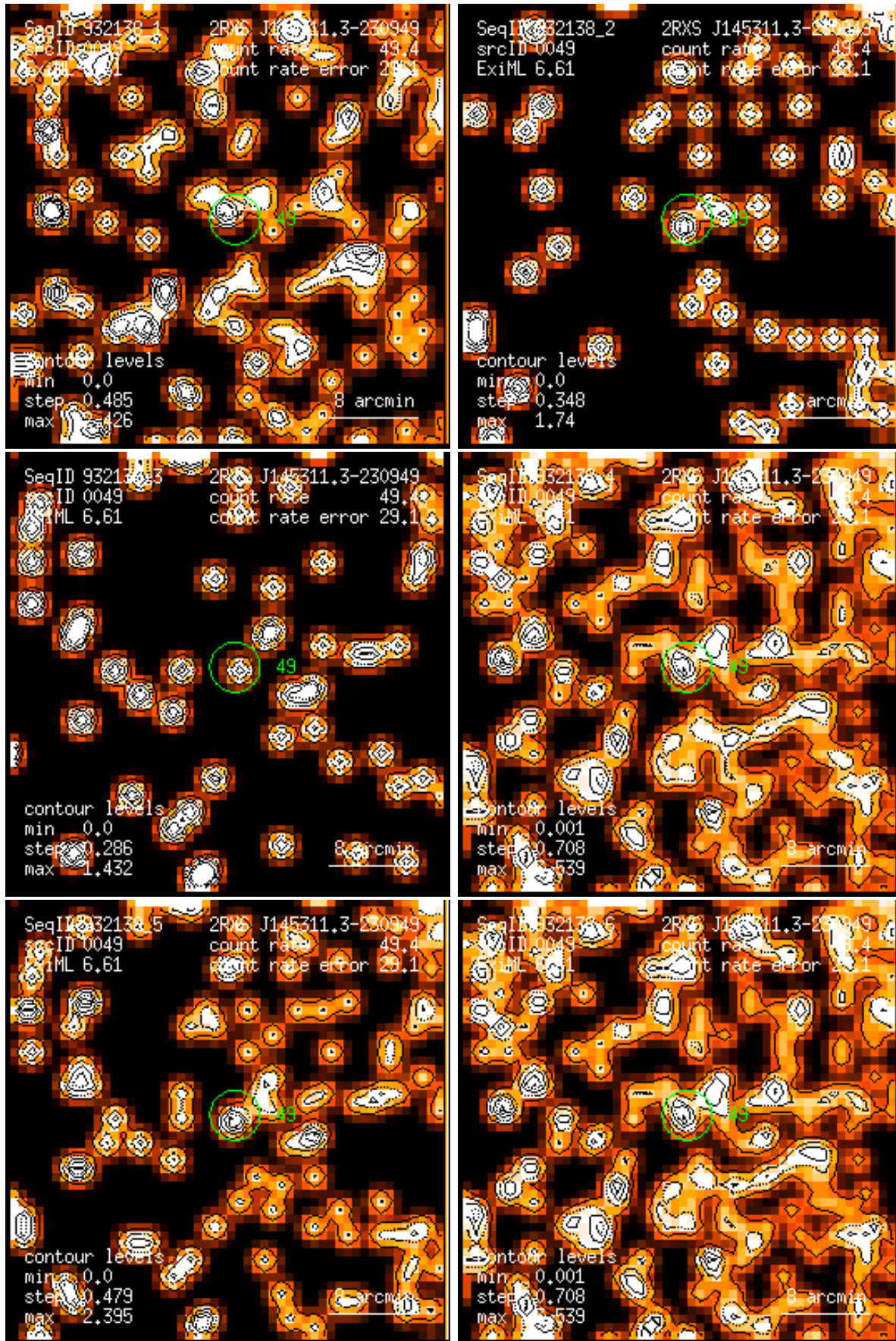
Figure 49: RASS 932138: detection 0049: band rate images, Gaussian filter: (1) PSPC channels 11 – 41, (2) 52 – 90, (3) 91 – 201, (4) 11 – 235, (5) 52 – 201, (6) 11 – 201. Broad band rates in counts/ks. Band rate contour levels in counts/ks/arcmin 2 .
