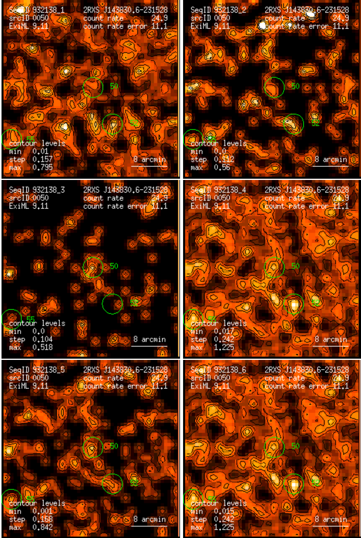
Figure 50: RASS 932138: detection 0050: band rate images, Gaussian filter: (1) PSPC channels 11 – 41, (2) 52 – 90, (3) 91 – 201, (4) 11 – 235, (5) 52 – 201, (6) 11 – 201. Broad band rates in counts/ks. Band rate contour levels in counts/ks/arcmin 2 .
