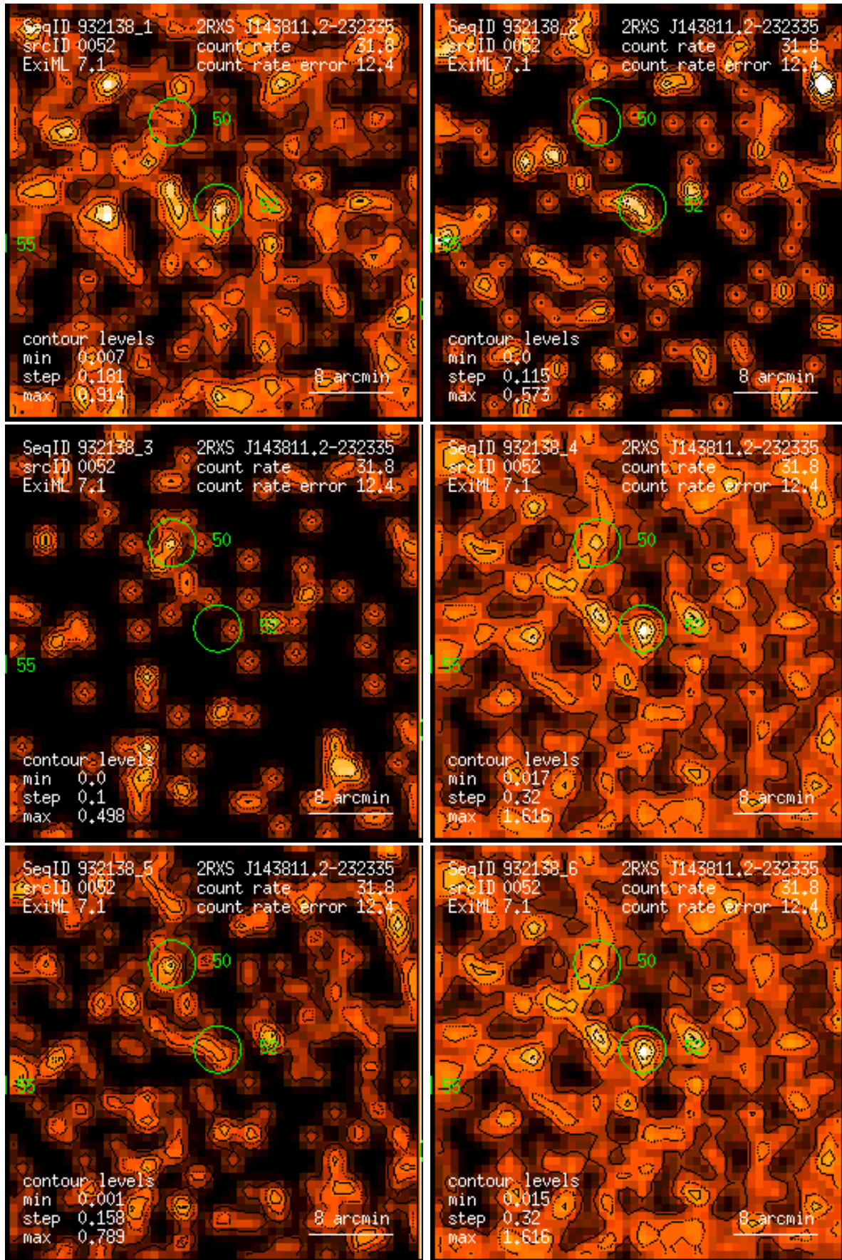
Figure 52: RASS 932138: detection 0052: band rate images, Gaussian filter: (1) PSPC channels 11 – 41, (2) 52 – 90, (3) 91 – 201, (4) 11 – 235, (5) 52 – 201, (6) 11 – 201. Broad band rates in counts/ks. Band rate contour levels in counts/ks/arcmin 2 .
