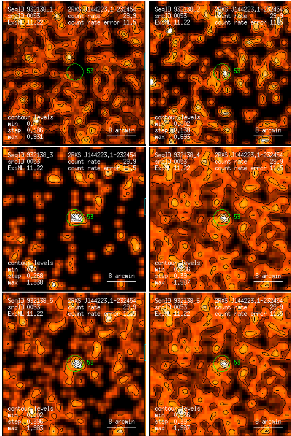
Figure 53: RASS 932138: detection 0053: band rate images, Gaussian filter: (1) PSPC channels 11 – 41, (2) 52 – 90, (3) 91 – 201, (4) 11 – 235, (5) 52 – 201, (6) 11 – 201. Broad band rates in counts/ks. Band rate contour levels in counts/ks/arcmin 2 .
