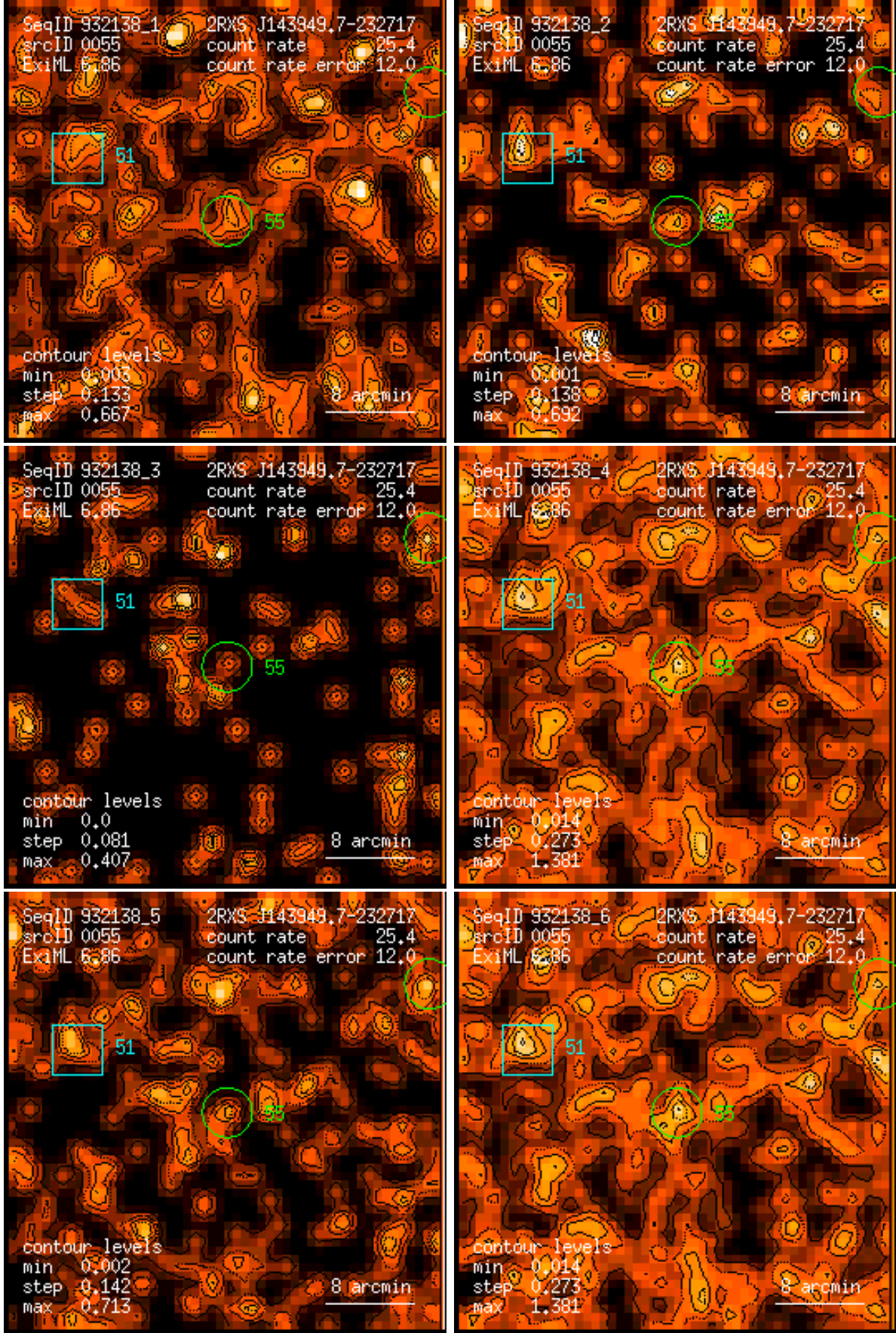
Figure 55: RASS 932138: detection 0055: band rate images, Gaussian filter: (1) PSPC channels 11 – 41, (2) 52 – 90, (3) 91 – 201, (4) 11 – 235, (5) 52 – 201, (6) 11 – 201. Broad band rates in counts/ks. Band rate contour levels in counts/ks/arcmin 2 .
