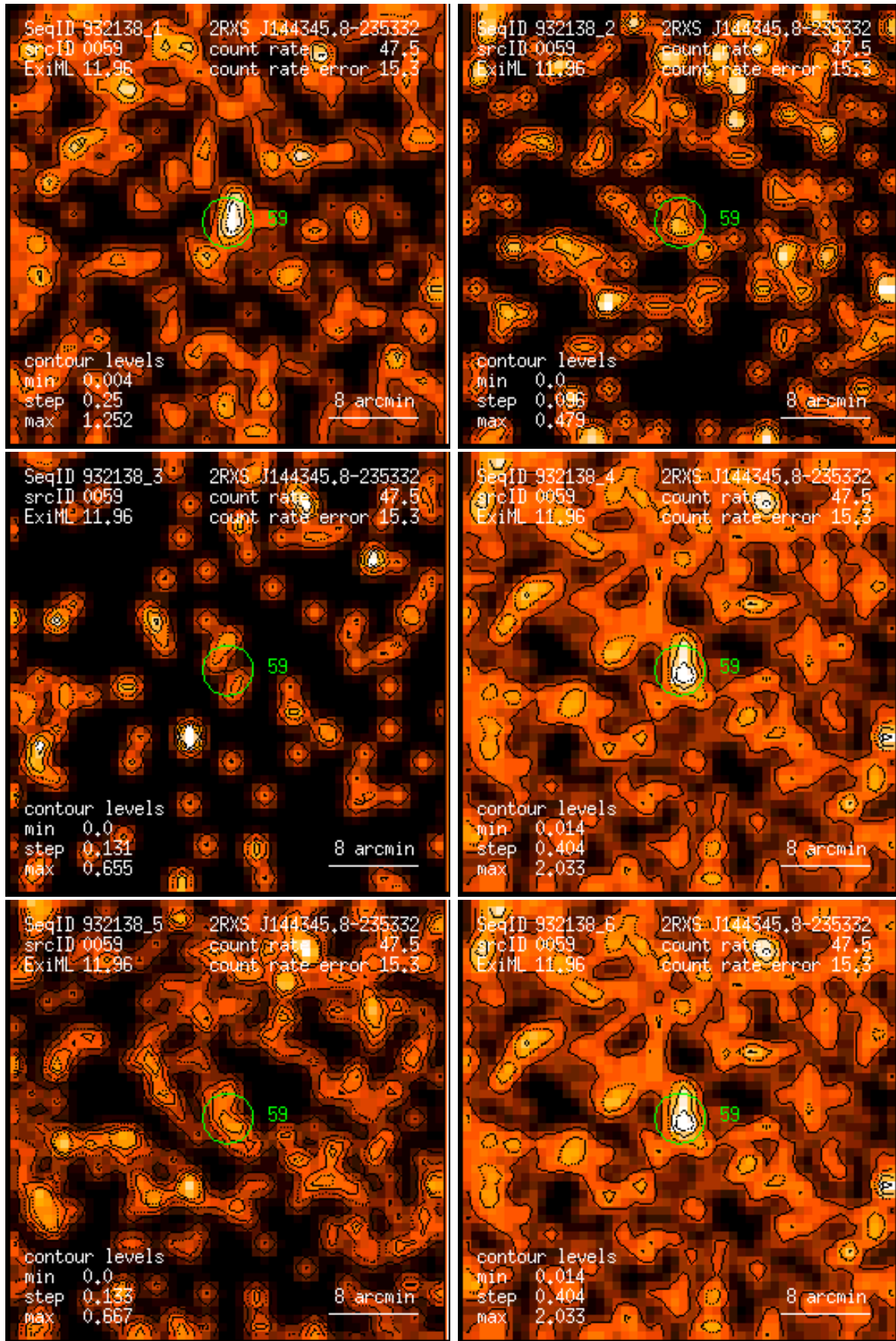
Figure 59: RASS 932138: detection 0059: band rate images, Gaussian filter: (1) PSPC channels 11 – 41, (2) 52 – 90, (3) 91 – 201, (4) 11 – 235, (5) 52 – 201, (6) 11 – 201. Broad band rates in counts/ks. Band rate contour levels in counts/ks/arcmin 2 .
