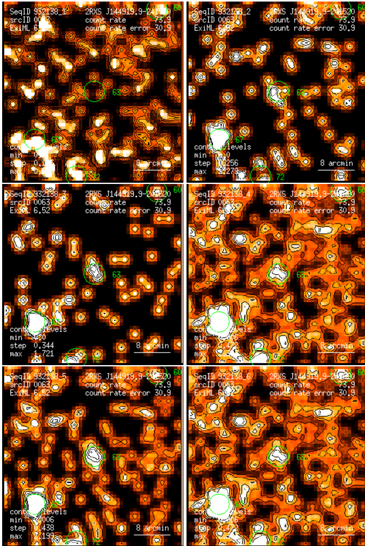
Figure 63: RASS 932138: detection 0063: band rate images, Gaussian filter: (1) PSPC channels 11 – 41, (2) 52 – 90, (3) 91 – 201, (4) 11 – 235, (5) 52 – 201, (6) 11 – 201. Broad band rates in counts/ks. Band rate contour levels in counts/ks/arcmin 2 .
