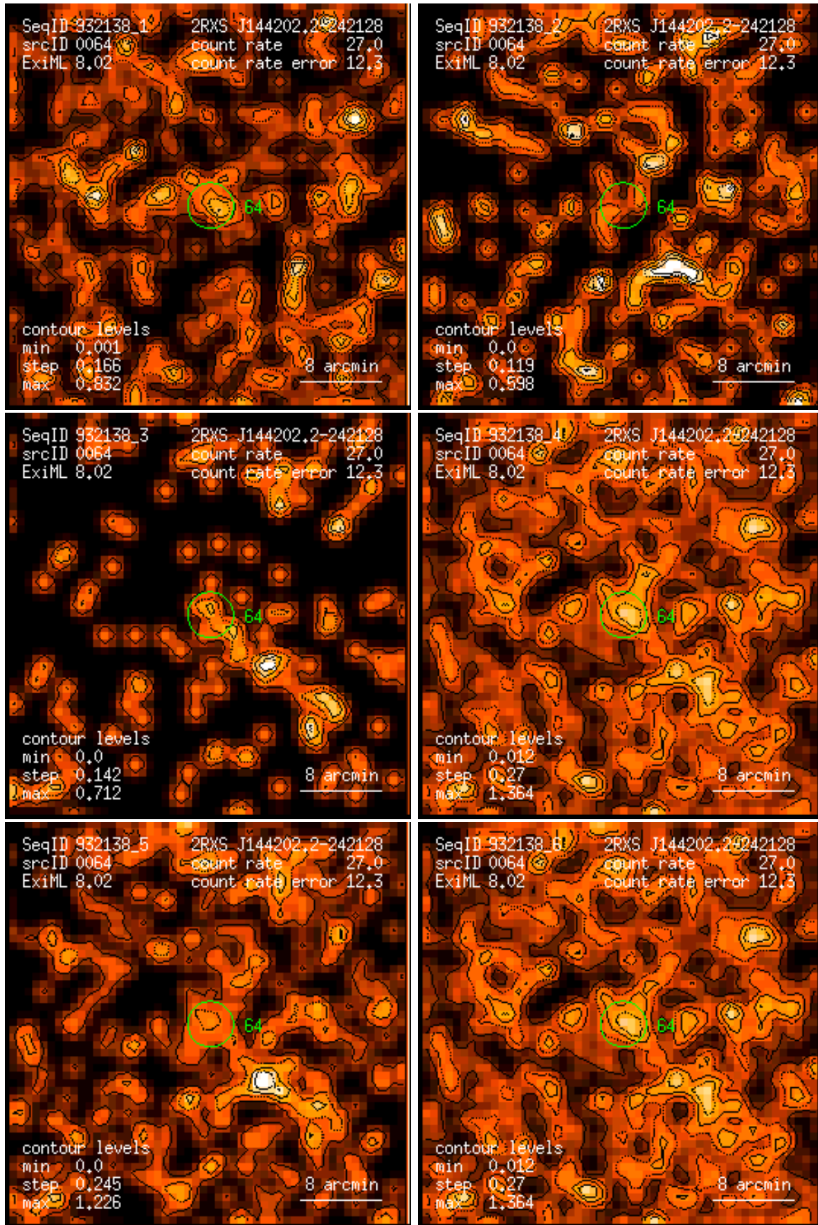
Figure 64: RASS 932138: detection 0064: band rate images, Gaussian filter: (1) PSPC channels 11 – 41, (2) 52 – 90, (3) 91 – 201, (4) 11 – 235, (5) 52 – 201, (6) 11 – 201. Broad band rates in counts/ks. Band rate contour levels in counts/ks/arcmin 2 .
