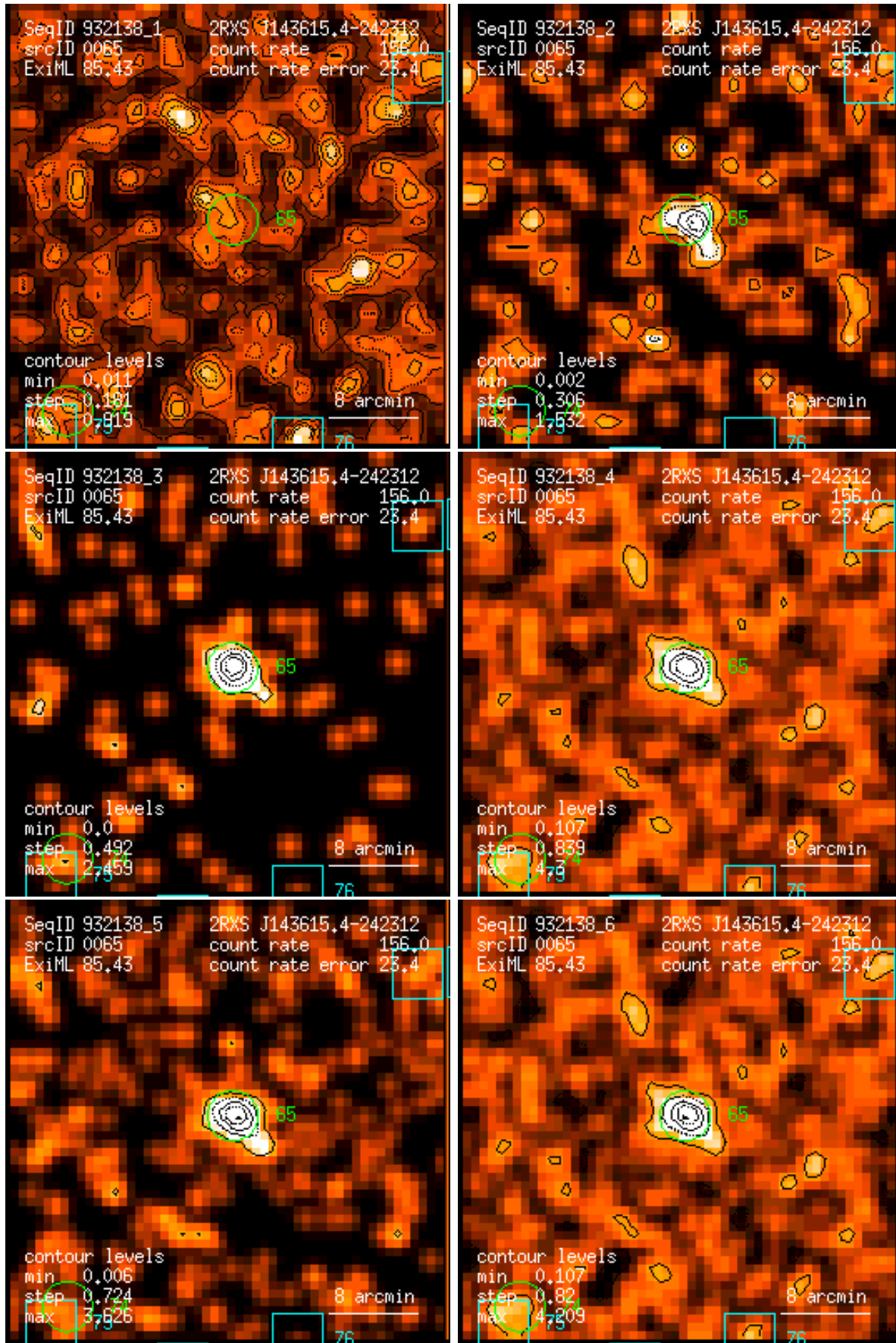
Figure 65: RASS 932138: detection 0065: band rate images, Gaussian filter: (1) PSPC channels 11 – 41, (2) 52 – 90, (3) 91 – 201, (4) 11 – 235, (5) 52 – 201, (6) 11 – 201. Broad band rates in counts/ks. Band rate contour levels in counts/ks/arcmin 2 .
