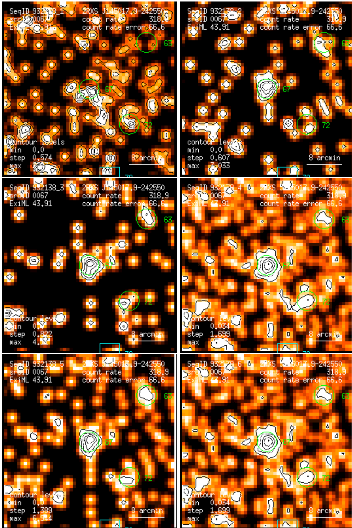
Figure 67: RASS 932138: detection 0067: band rate images, Gaussian filter: (1) PSPC channels 11 – 41, (2) 52 – 90, (3) 91 – 201, (4) 11 – 235, (5) 52 – 201, (6) 11 – 201. Broad band rates in counts/ks. Band rate contour levels in counts/ks/arcmin 2 .
