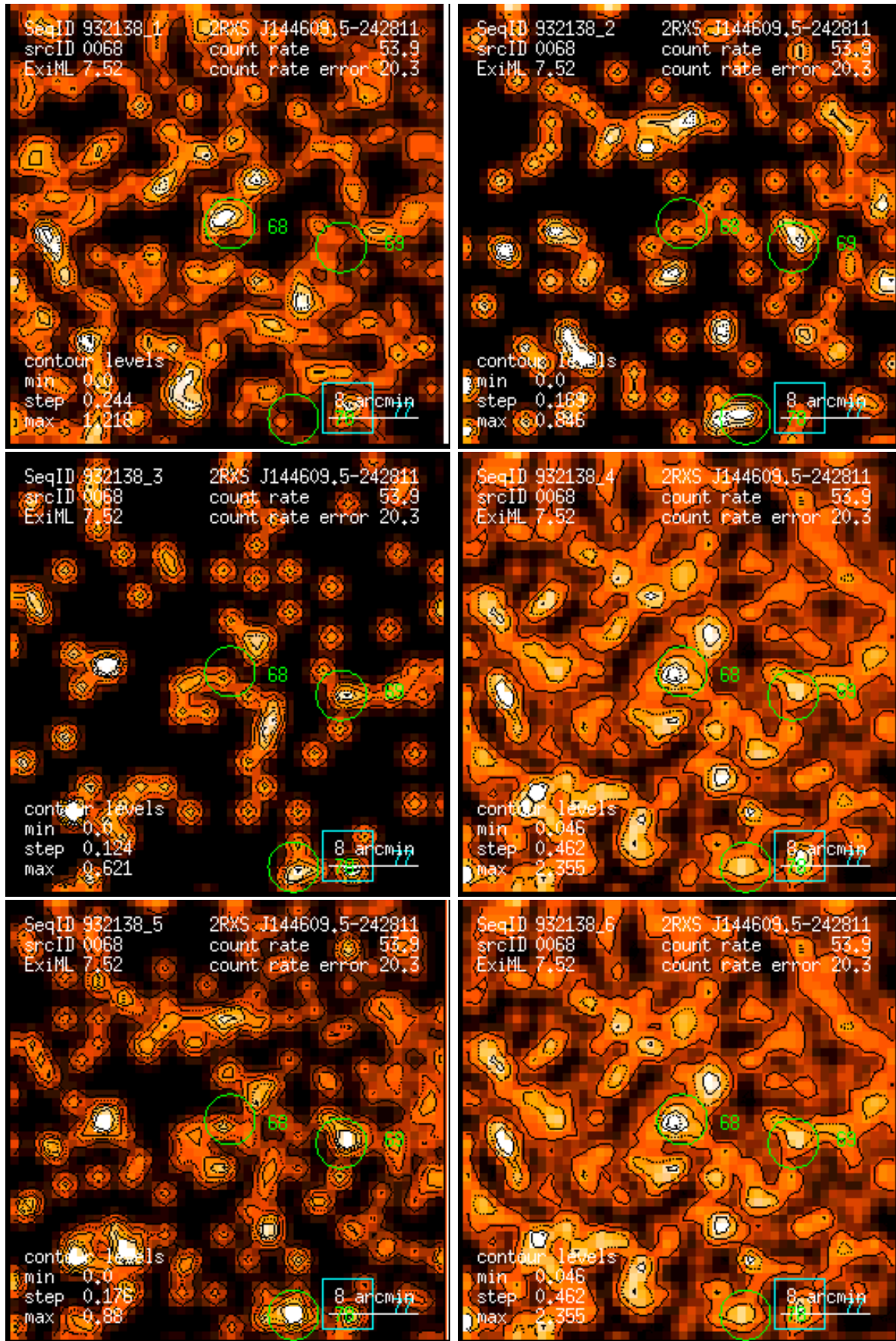
Figure 68: RASS 932138: detection 0068: band rate images, Gaussian filter: (1) PSPC channels 11 – 41, (2) 52 – 90, (3) 91 – 201, (4) 11 – 235, (5) 52 – 201, (6) 11 – 201. Broad band rates in counts/ks. Band rate contour levels in counts/ks/arcmin 2 .
