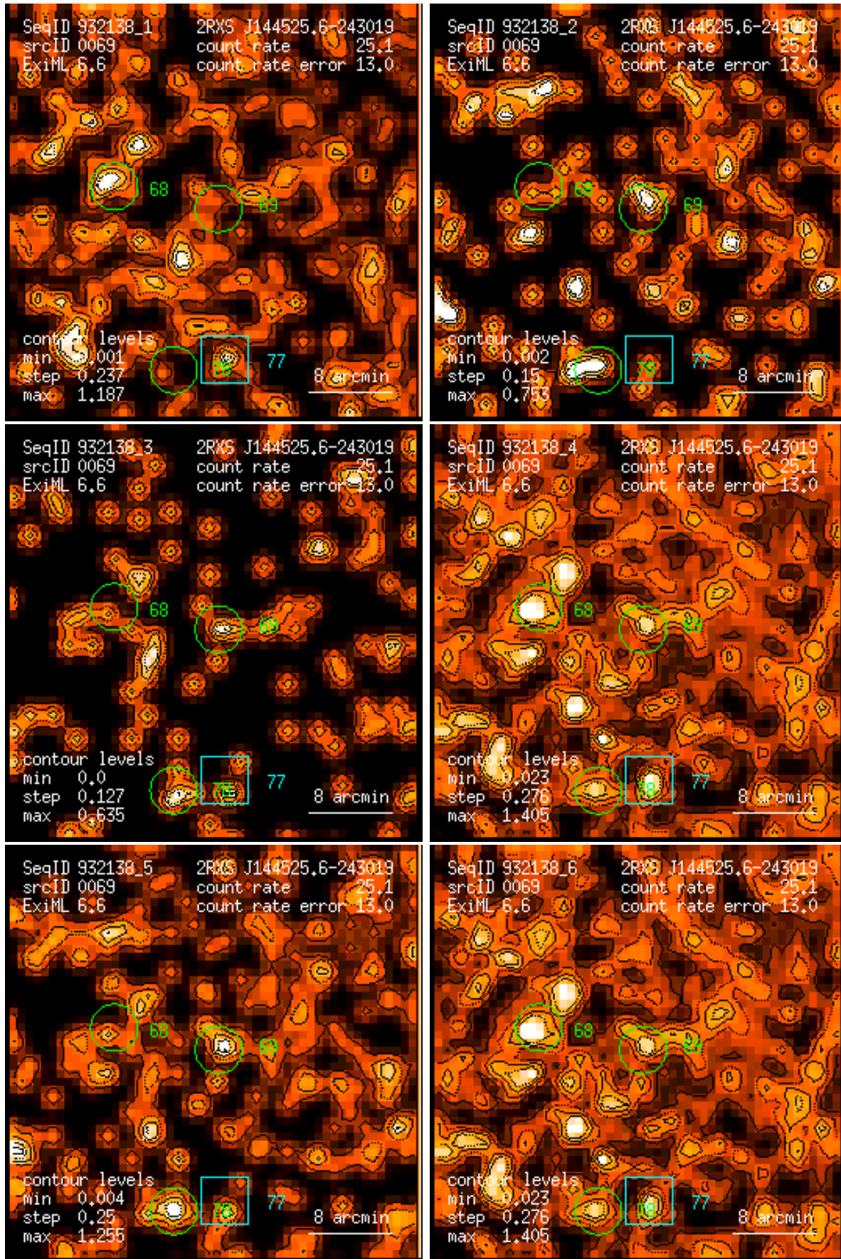
Figure 69: RASS 932138: detection 0069: band rate images, Gaussian filter: (1) PSPC channels 11 – 41, (2) 52 – 90, (3) 91 – 201, (4) 11 – 235, (5) 52 – 201, (6) 11 – 201. Broad band rates in counts/ks. Band rate contour levels in counts/ks/arcmin 2 .
