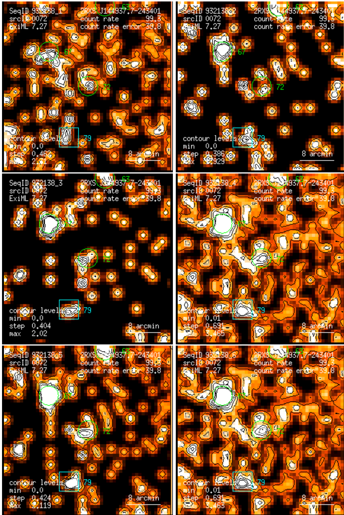
Figure 72: RASS 932138: detection 0072: band rate images, Gaussian filter: (1) PSPC channels 11 – 41, (2) 52 – 90, (3) 91 – 201, (4) 11 – 235, (5) 52 – 201, (6) 11 – 201. Broad band rates in counts/ks. Band rate contour levels in counts/ks/arcmin 2 .
