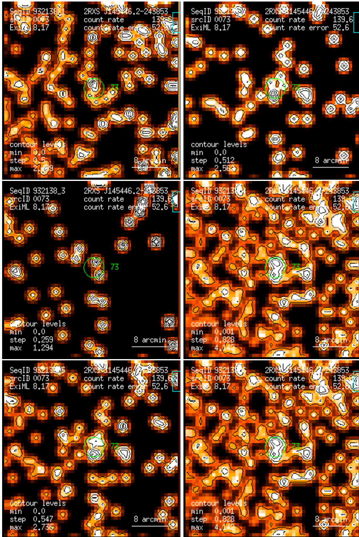
Figure 73: RASS 932138: detection 0073: band rate images, Gaussian filter: (1) PSPC channels 11 – 41, (2) 52 – 90, (3) 91 – 201, (4) 11 – 235, (5) 52 – 201, (6) 11 – 201. Broad band rates in counts/ks. Band rate contour levels in counts/ks/arcmin 2 .
