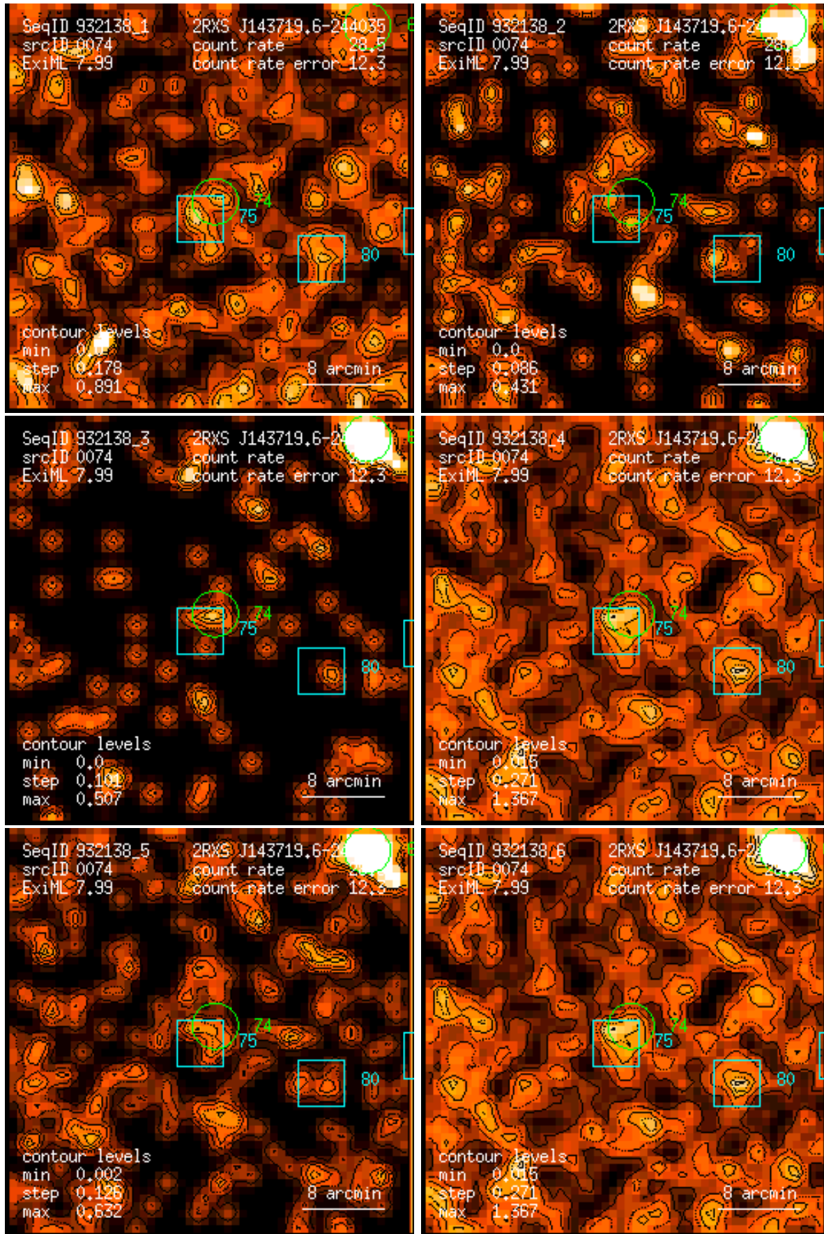
Figure 74: RASS 932138: detection 0074: band rate images, Gaussian filter: (1) PSPC channels 11 – 41, (2) 52 – 90, (3) 91 – 201, (4) 11 – 235, (5) 52 – 201, (6) 11 – 201. Broad band rates in counts/ks. Band rate contour levels in counts/ks/arcmin 2 .
