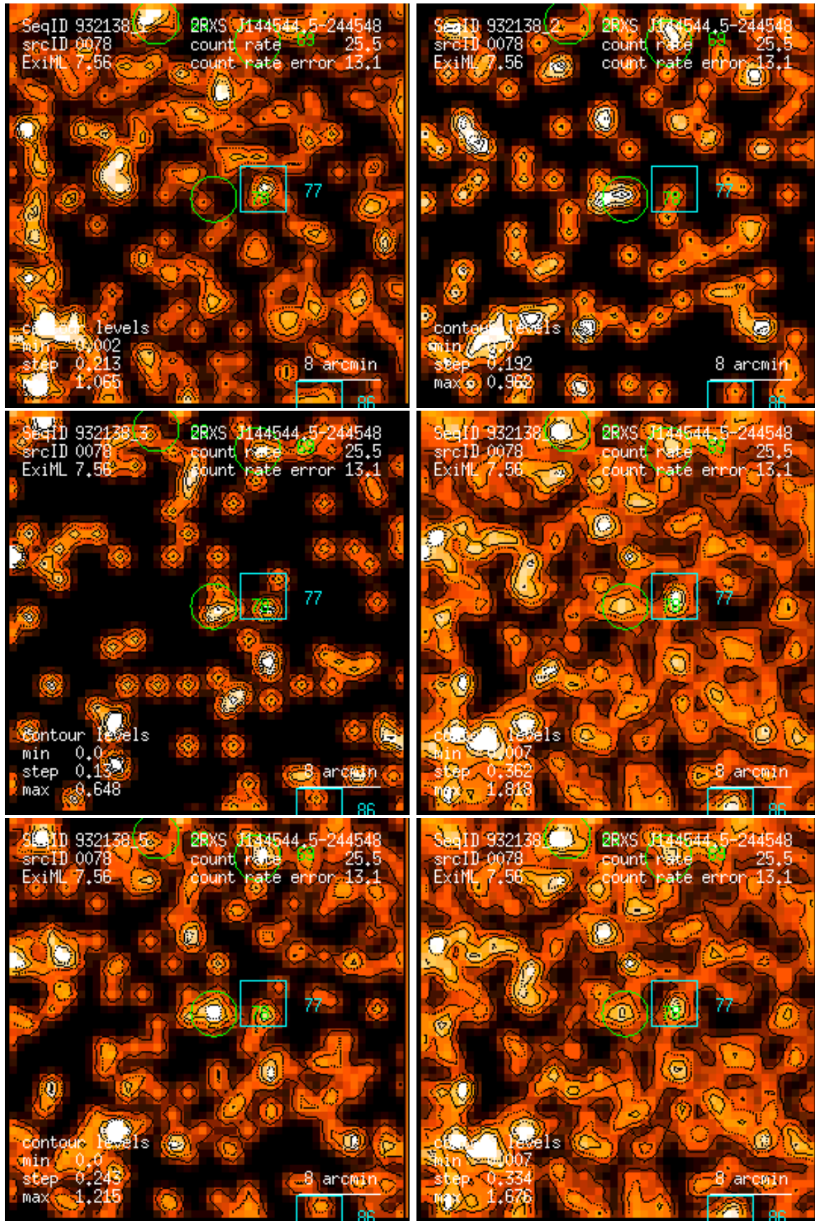
Figure 78: RASS 932138: detection 0078: band rate images, Gaussian filter: (1) PSPC channels 11 – 41, (2) 52 – 90, (3) 91 – 201, (4) 11 – 235, (5) 52 – 201, (6) 11 – 201. Broad band rates in counts/ks. Band rate contour levels in counts/ks/arcmin 2 .
