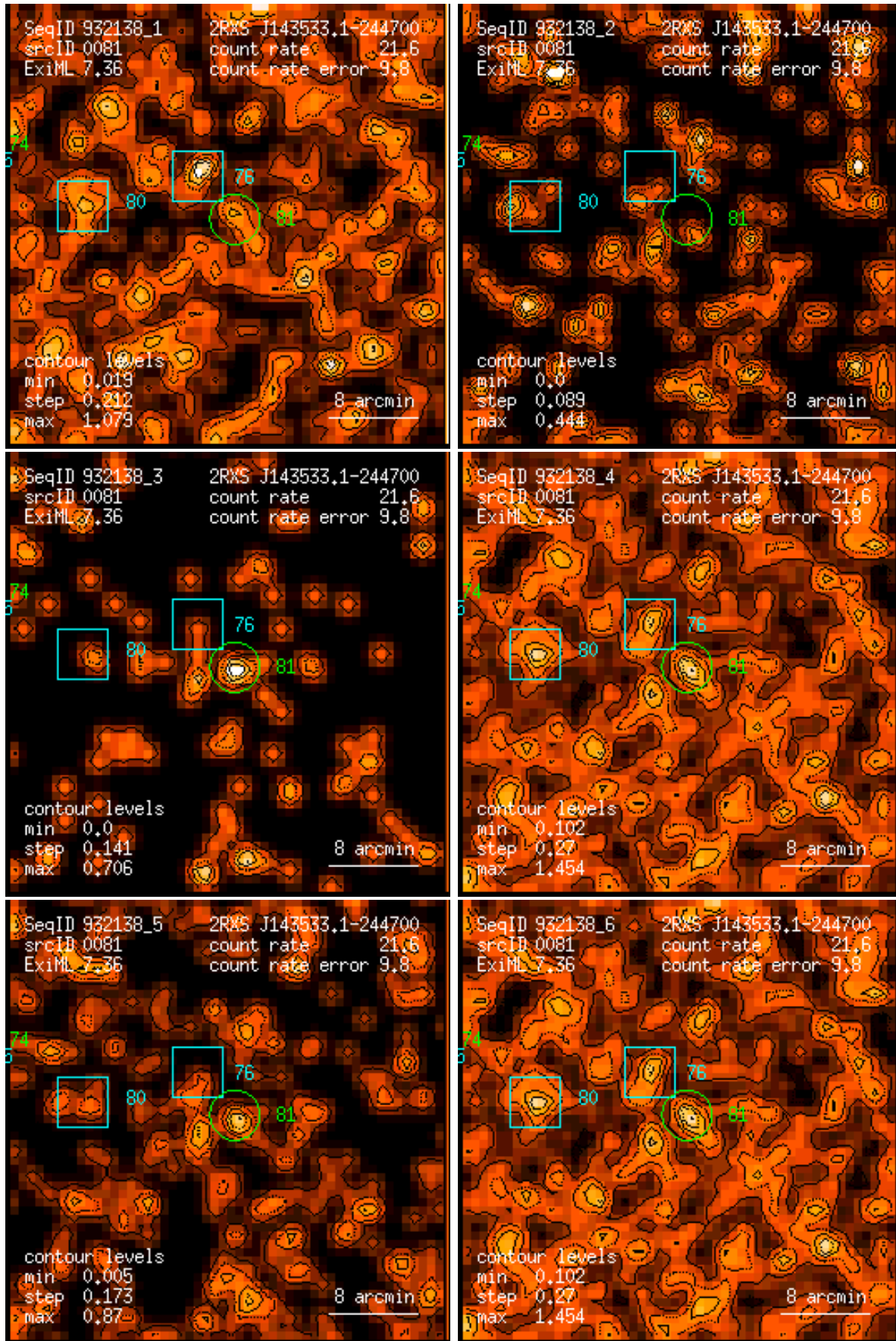
Figure 81: RASS 932138: detection 0081: band rate images, Gaussian filter: (1) PSPC channels 11 – 41, (2) 52 – 90, (3) 91 – 201, (4) 11 – 235, (5) 52 – 201, (6) 11 – 201. Broad band rates in counts/ks. Band rate contour levels in counts/ks/arcmin 2 .
