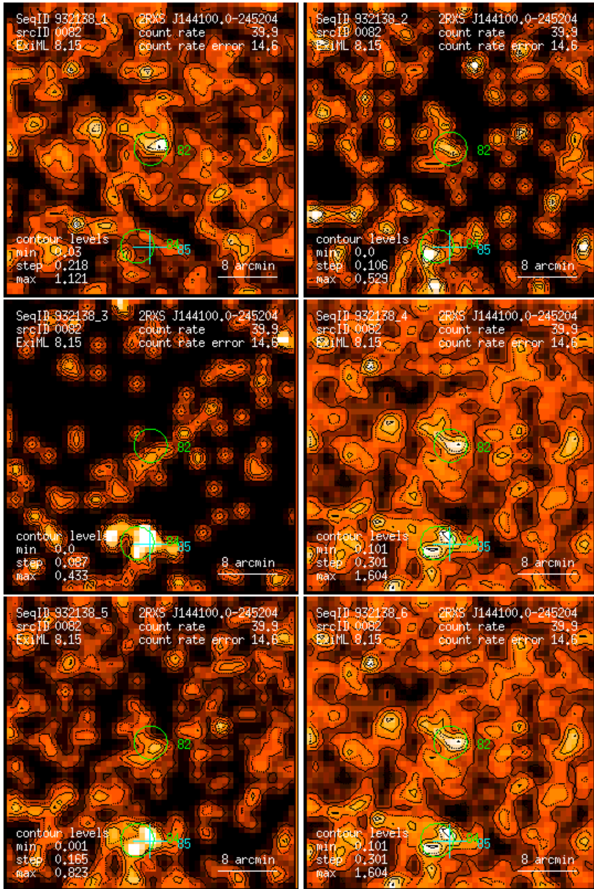
Figure 82: RASS 932138: detection 0082: band rate images, Gaussian filter: (1) PSPC channels 11 – 41, (2) 52 – 90, (3) 91 – 201, (4) 11 – 235, (5) 52 – 201, (6) 11 – 201. Broad band rates in counts/ks. Band rate contour levels in counts/ks/arcmin 2 .
