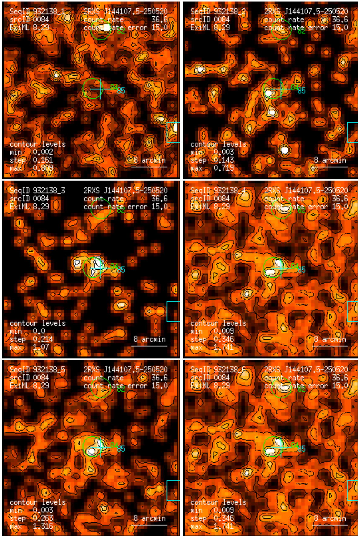
Figure 84: RASS 932138: detection 0084: band rate images, Gaussian filter: (1) PSPC channels 11 – 41, (2) 52 – 90, (3) 91 – 201, (4) 11 – 235, (5) 52 – 201, (6) 11 – 201. Broad band rates in counts/ks. Band rate contour levels in counts/ks/arcmin 2 .
